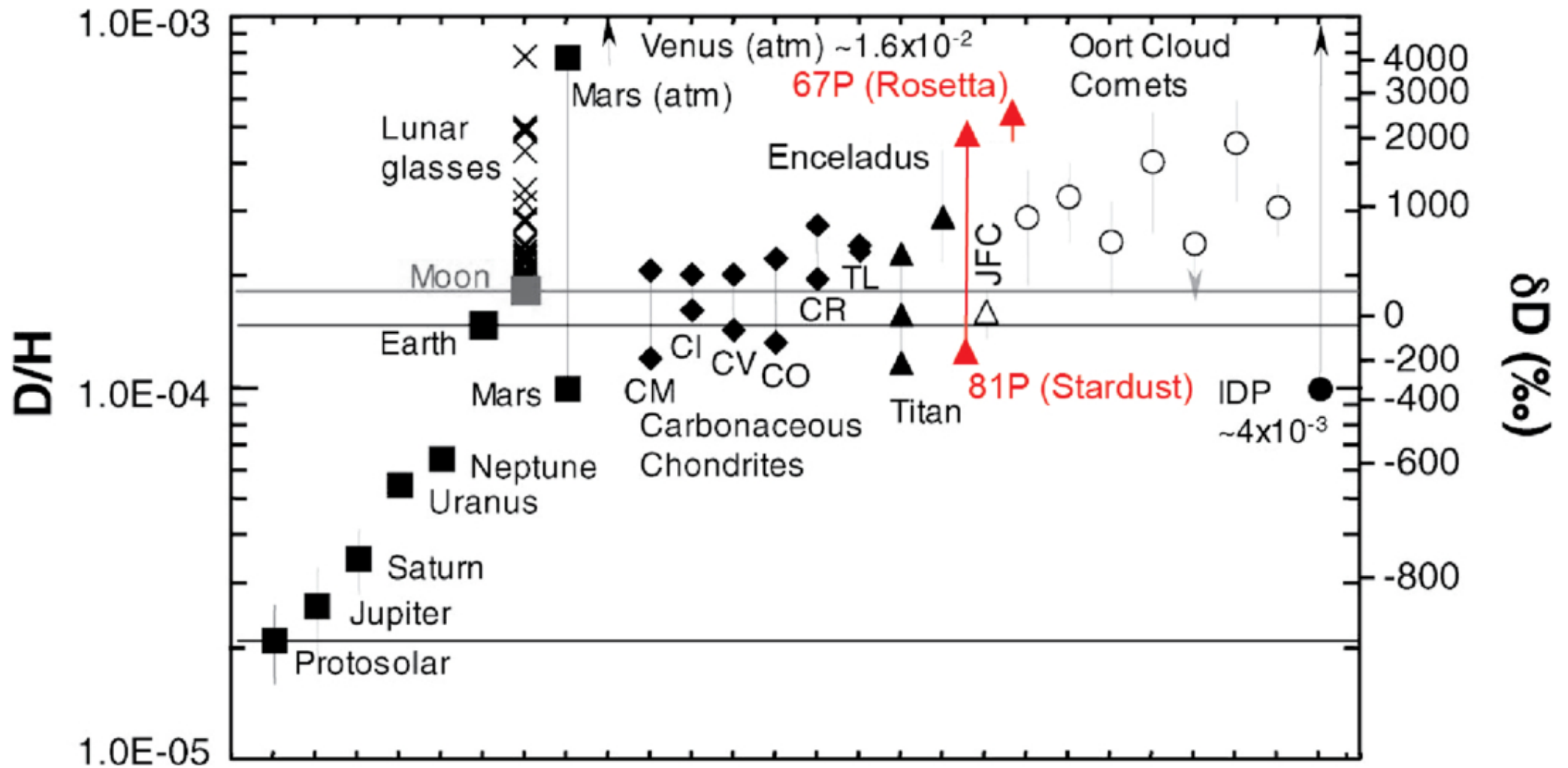
Figure 3. from Mallory J. Kinczyk et al 2026 Planet. Sci. J. 7 doi:10.3847/PSJ/ae771f https://dx.doi.org/10.3847/PSJ/ae771f © 2026. The Author(s). Published by the American Astronomical Society.
