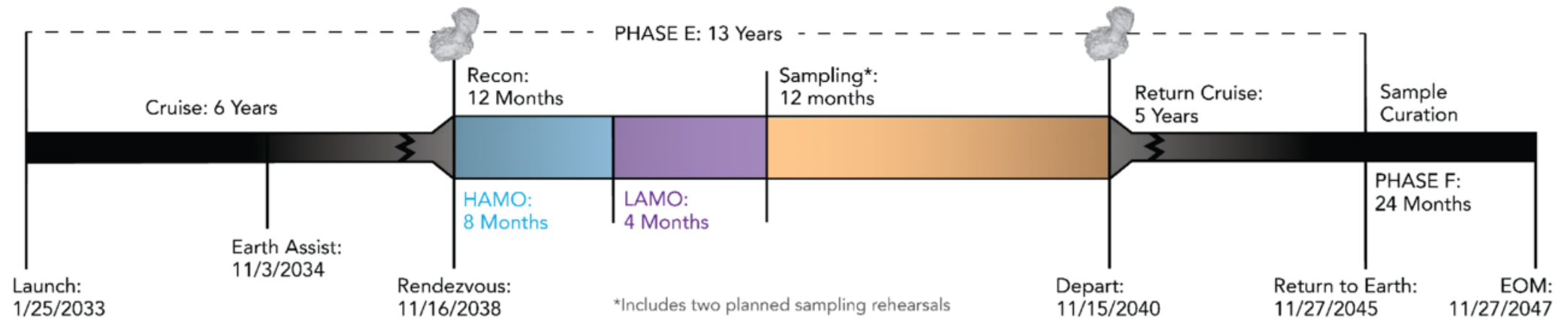
Figure 1. from Mallory J. Kinczyk et al 2026 Planet. Sci. J. 7 doi:10.3847/PSJ/ae771f https://dx.doi.org/10.3847/PSJ/ae771f © 2026. The Author(s). Published by the American Astronomical Society.
