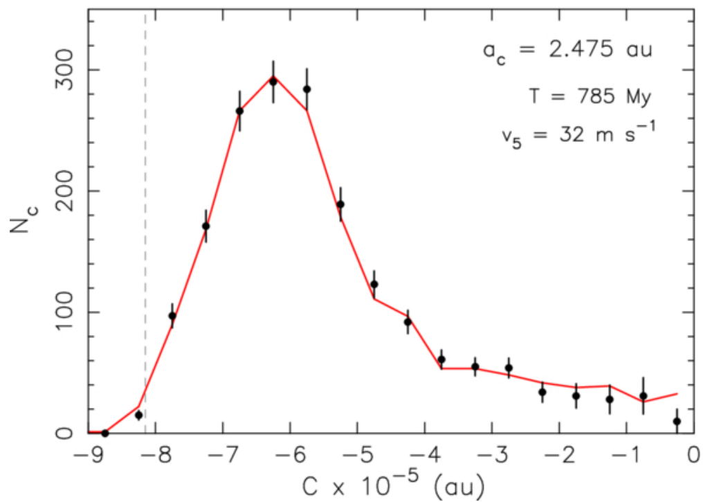
Figure 7. from William F. Bottke et al 2026 Planet. Sci. J. 7 doi:10.3847/PSJ/ae74cc https://dx.doi.org/10.3847/PSJ/ae74cc © 2026. The Author(s). Published by the American Astronomical Society.
