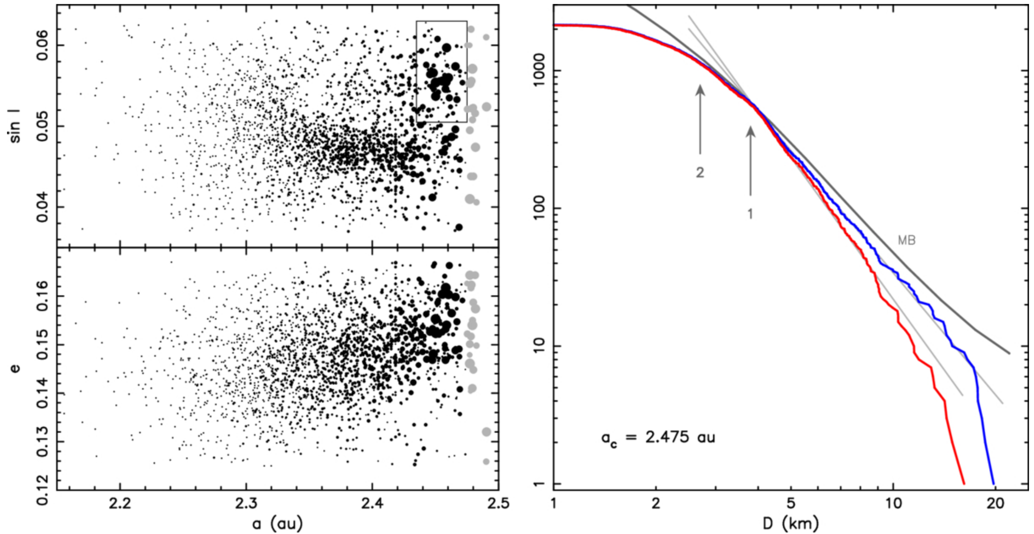
Figure 6. from William F. Bottke et al 2026 Planet. Sci. J. 7 doi:10.3847/PSJ/ae74cc https://dx.doi.org/10.3847/PSJ/ae74cc © 2026. The Author(s). Published by the American Astronomical Society.
