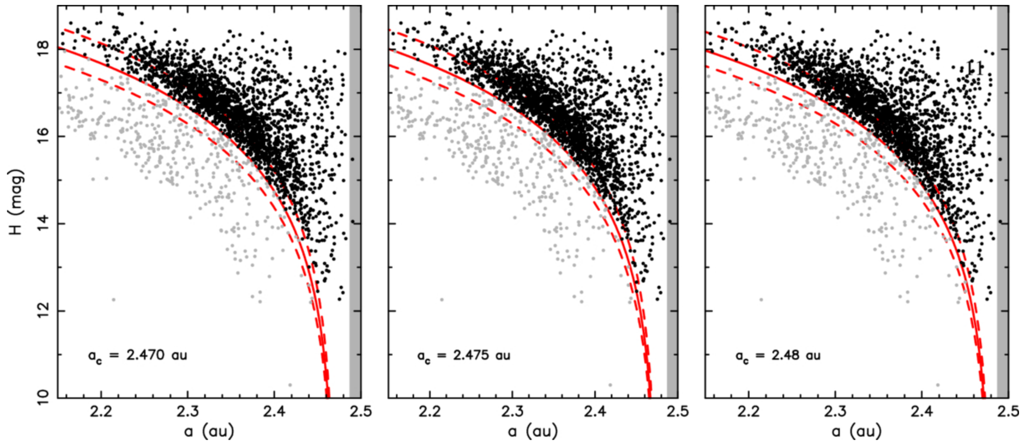
Figure 5. from William F. Bottke et al 2026 Planet. Sci. J. 7 doi:10.3847/PSJ/ae74cc https://dx.doi.org/10.3847/PSJ/ae74cc © 2026. The Author(s). Published by the American Astronomical Society.
