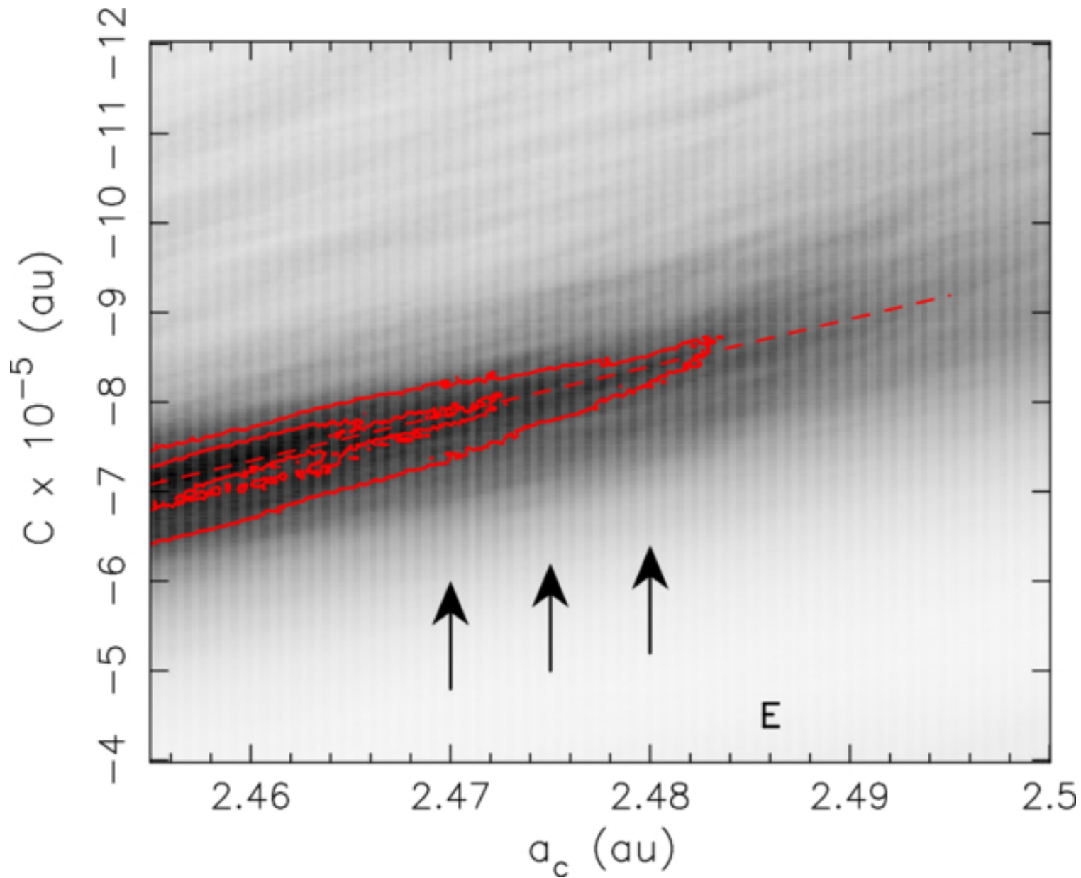
Figure 4. from William F. Bottke et al 2026 Planet. Sci. J. 7 doi:10.3847/PSJ/ae74cc https://dx.doi.org/10.3847/PSJ/ae74cc © 2026. The Author(s). Published by the American Astronomical Society.
