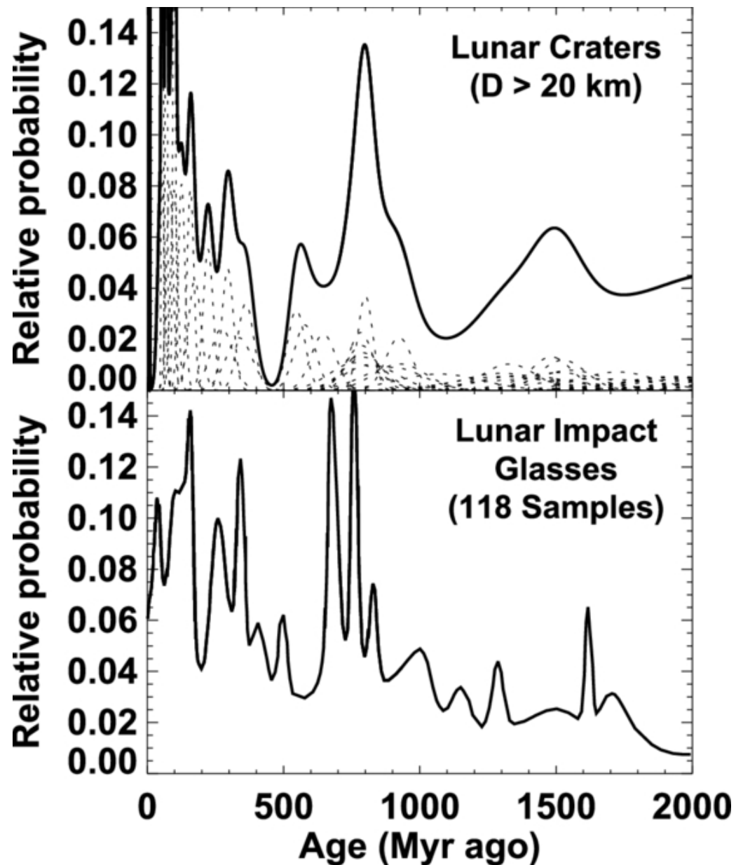
Figure 3. from William F. Bottke et al 2026 Planet. Sci. J. 7 doi:10.3847/PSJ/ae74cc https://dx.doi.org/10.3847/PSJ/ae74cc © 2026. The Author(s). Published by the American Astronomical Society.
