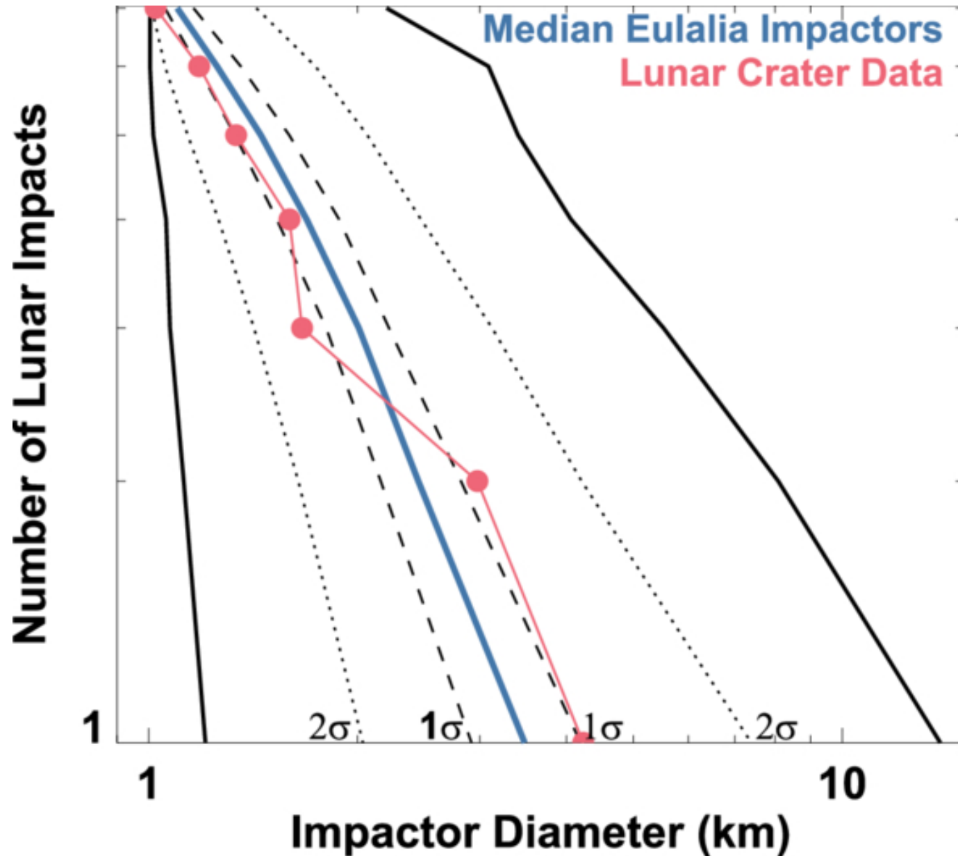
Figure 18. from William F. Bottke et al 2026 Planet. Sci. J. 7 doi:10.3847/PSJ/ae74cc https://dx.doi.org/10.3847/PSJ/ae74cc © 2026. The Author(s). Published by the American Astronomical Society.
