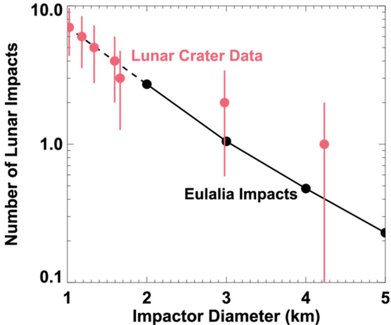
Figure 17. from William F. Bottke et al 2026 Planet. Sci. J. 7 doi:10.3847/PSJ/ae74cc https://dx.doi.org/10.3847/PSJ/ae74cc © 2026. The Author(s). Published by the American Astronomical Society.
