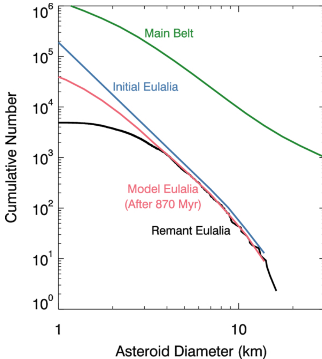
Figure 14. from William F. Bottke et al 2026 Planet. Sci. J. 7 doi:10.3847/PSJ/ae74cc https://dx.doi.org/10.3847/PSJ/ae74cc © 2026. The Author(s). Published by the American Astronomical Society.
