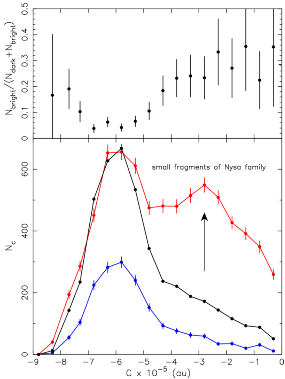
Figure 13. from William F. Bottke et al 2026 Planet. Sci. J. 7 doi:10.3847/PSJ/ae74cc https://dx.doi.org/10.3847/PSJ/ae74cc © 2026. The Author(s). Published by the American Astronomical Society.
