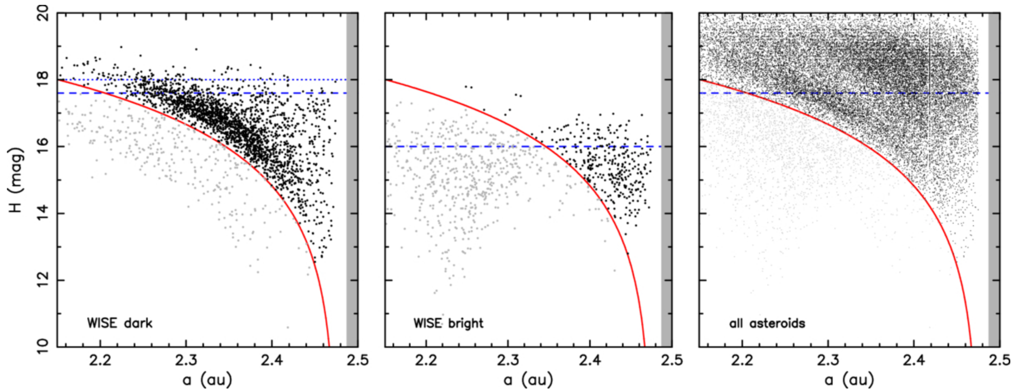
Figure 12. from William F. Bottke et al 2026 Planet. Sci. J. 7 doi:10.3847/PSJ/ae74cc https://dx.doi.org/10.3847/PSJ/ae74cc © 2026. The Author(s). Published by the American Astronomical Society.
