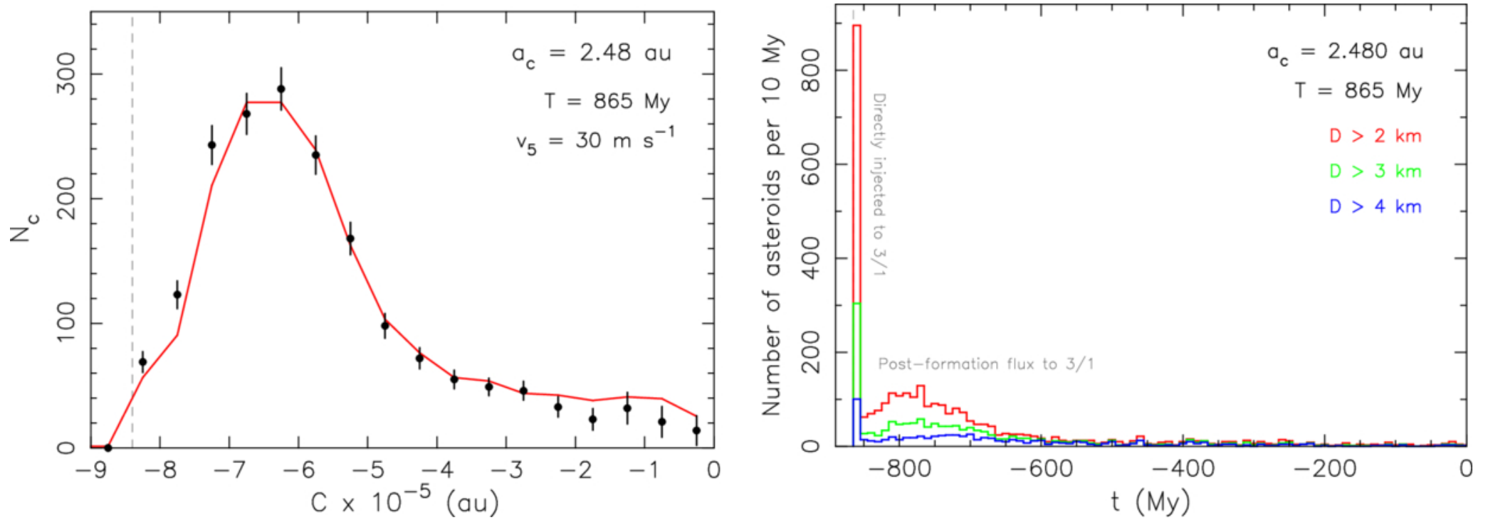
Figure 11. from William F. Bottke et al 2026 Planet. Sci. J. 7 doi:10.3847/PSJ/ae74cc https://dx.doi.org/10.3847/PSJ/ae74cc © 2026. The Author(s). Published by the American Astronomical Society.
