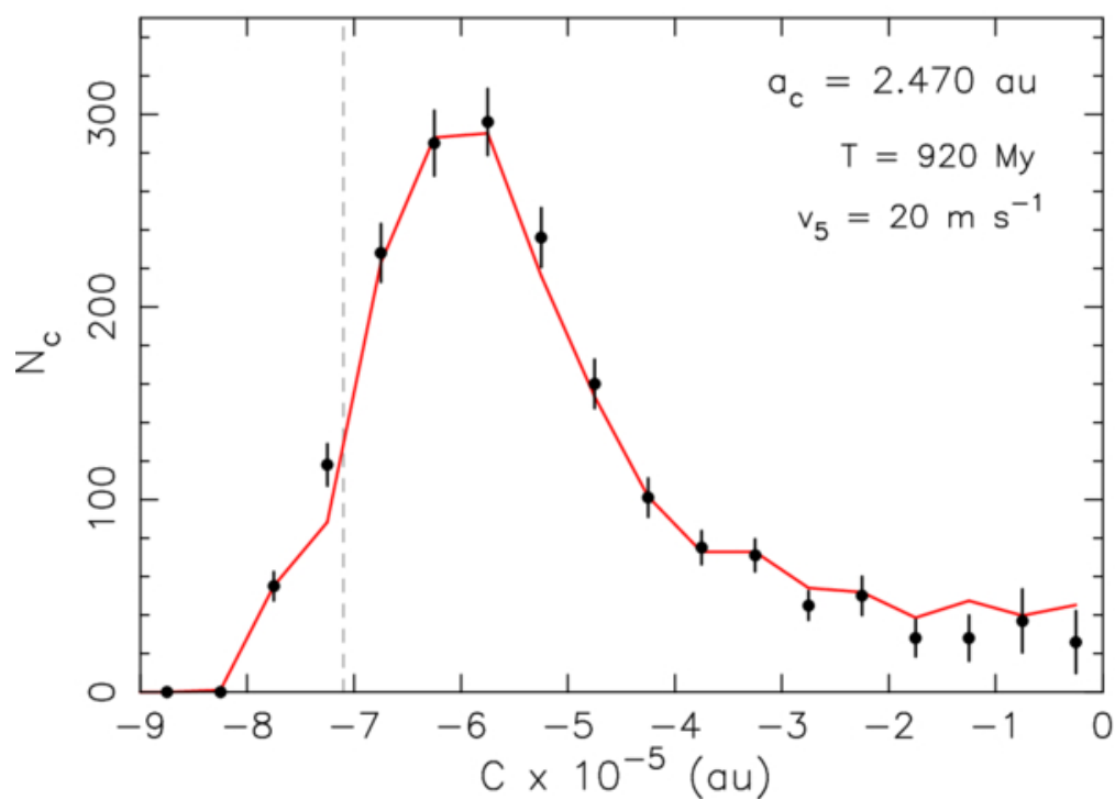
Figure 10. from William F. Bottke et al 2026 Planet. Sci. J. 7 doi:10.3847/PSJ/ae74cc https://dx.doi.org/10.3847/PSJ/ae74cc © 2026. The Author(s). Published by the American Astronomical Society.
