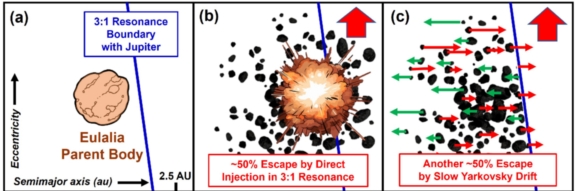
Figure 1. from William F. Bottke et al 2026 Planet. Sci. J. 7 doi:10.3847/PSJ/ae74cc https://dx.doi.org/10.3847/PSJ/ae74cc © 2026. The Author(s). Published by the American Astronomical Society.
