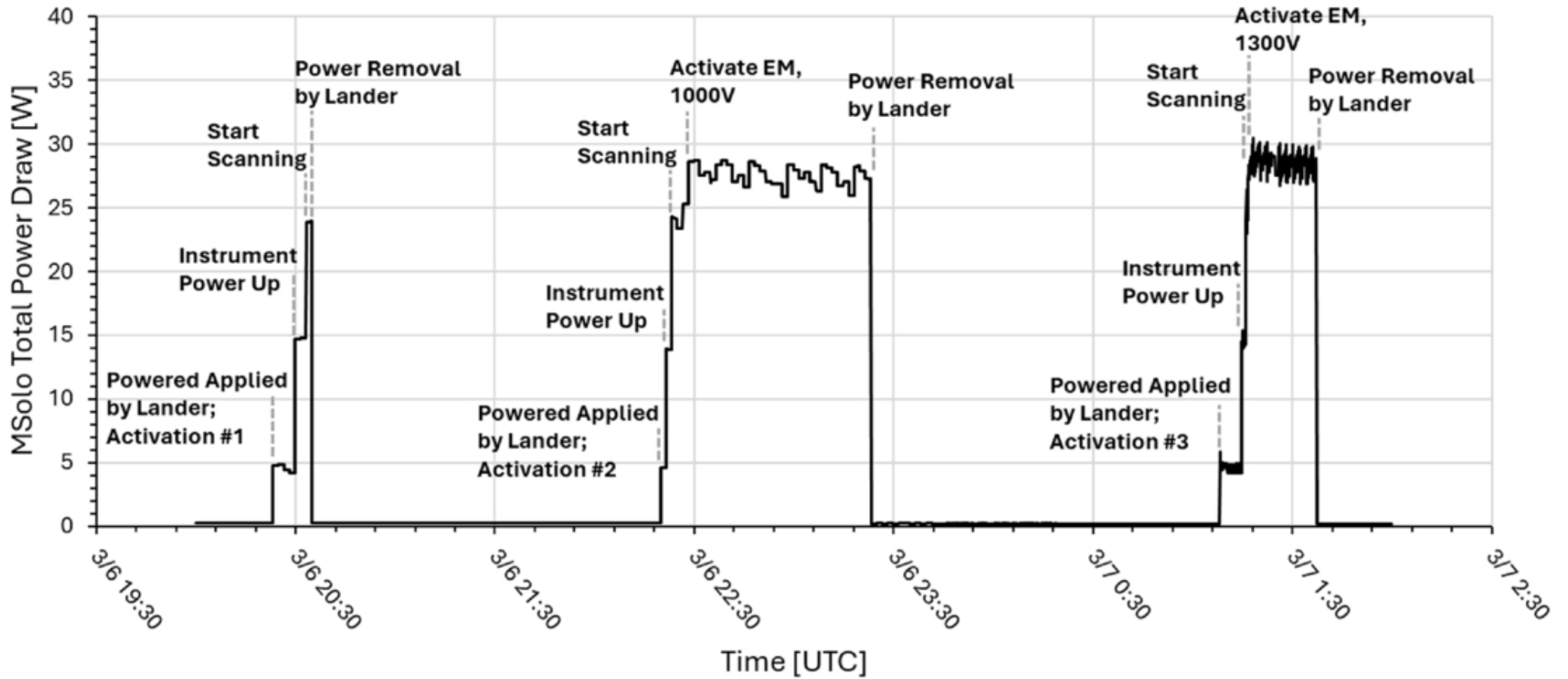
Figure 24. from Matthew Hancock et al 2026 Planet. Sci. J. 7 doi:10.3847/PSJ/ae732f https://dx.doi.org/10.3847/PSJ/ae732f © 2026. The Author(s). Published by the American Astronomical Society.
