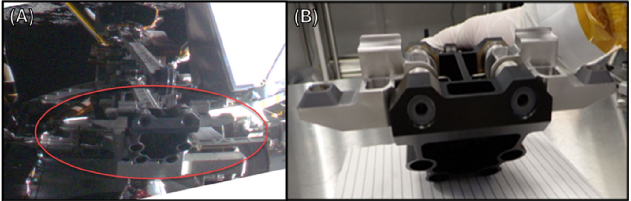
Figure 23. from Matthew Hancock et al 2026 Planet. Sci. J. 7 doi:10.3847/PSJ/ae732f https://dx.doi.org/10.3847/PSJ/ae732f © 2026. The Author(s). Published by the American Astronomical Society.
