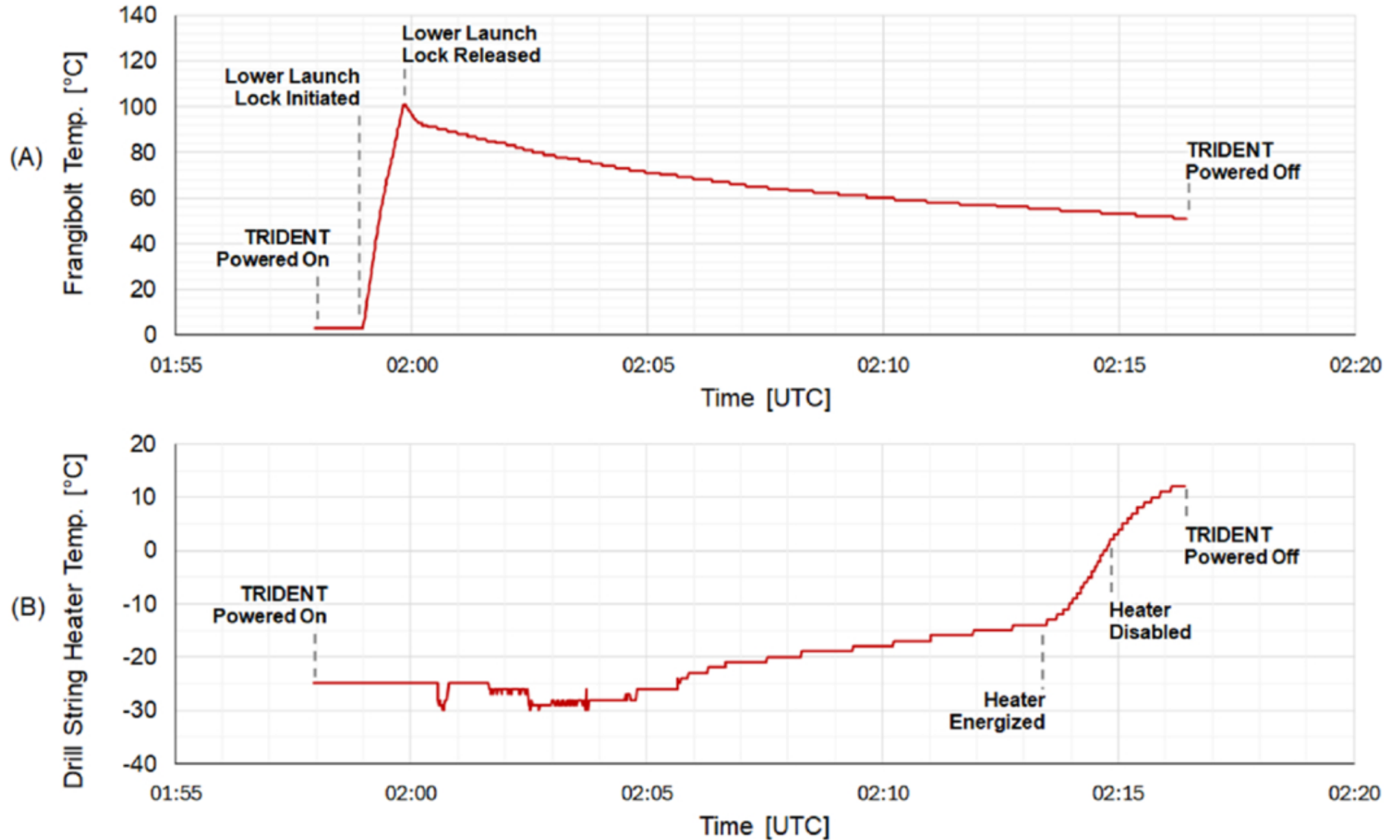
Figure 22. from Matthew Hancock et al 2026 Planet. Sci. J. 7 doi:10.3847/PSJ/ae732f https://dx.doi.org/10.3847/PSJ/ae732f © 2026. The Author(s). Published by the American Astronomical Society.
