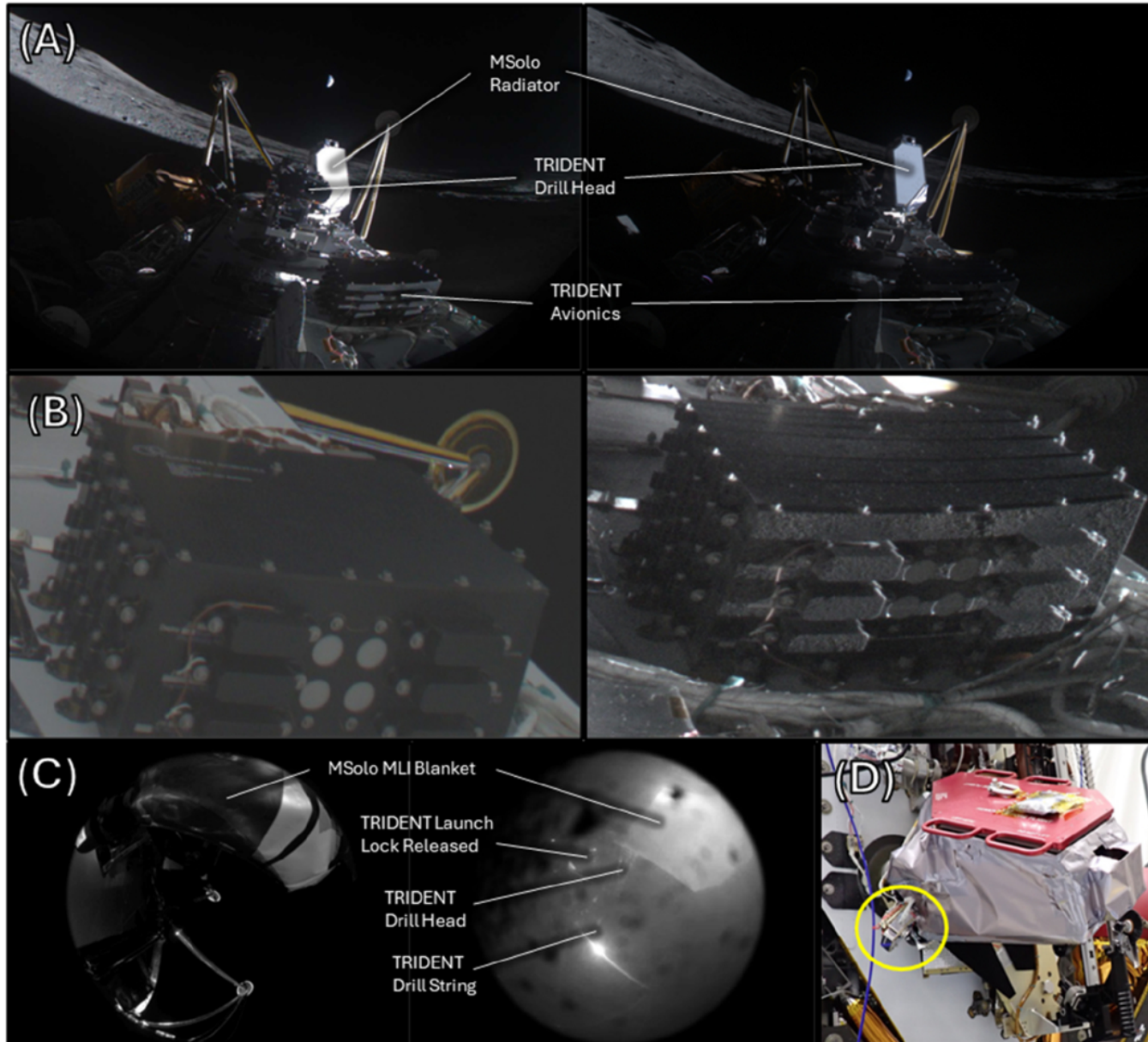
Figure 20. from Matthew Hancock et al 2026 Planet. Sci. J. 7 doi:10.3847/PSJ/ae732f https://dx.doi.org/10.3847/PSJ/ae732f © 2026. The Author(s). Published by the American Astronomical Society.
