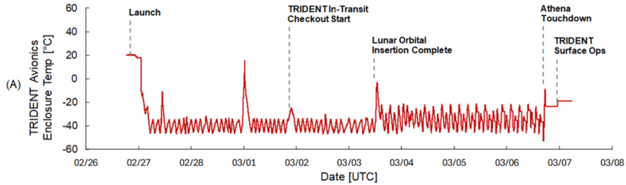
Figure 16. from Matthew Hancock et al 2026 Planet. Sci. J. 7 doi:10.3847/PSJ/ae732f https://dx.doi.org/10.3847/PSJ/ae732f © 2026. The Author(s). Published by the American Astronomical Society.
