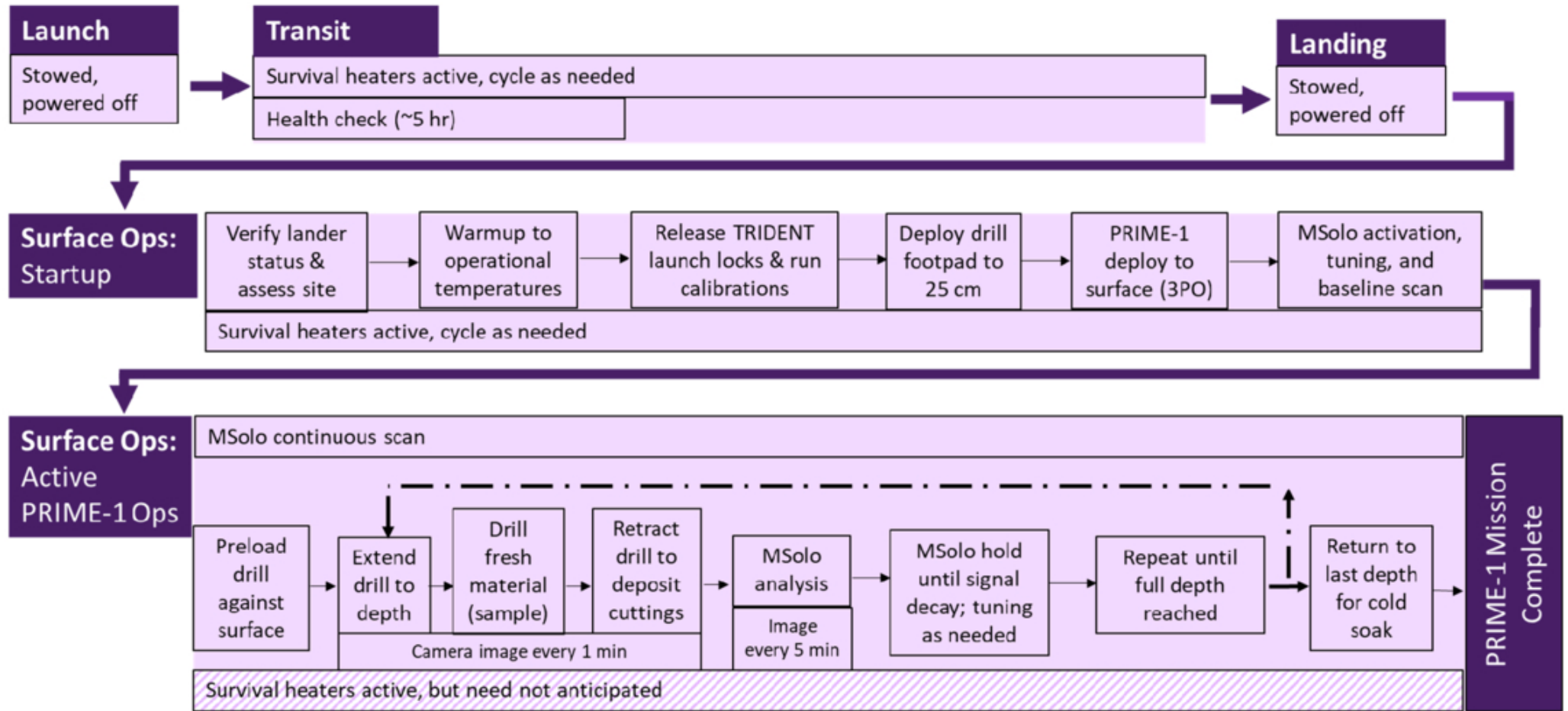
Figure 10. from Matthew Hancock et al 2026 Planet. Sci. J. 7 doi:10.3847/PSJ/ae732f https://dx.doi.org/10.3847/PSJ/ae732f © 2026. The Author(s). Published by the American Astronomical Society.
