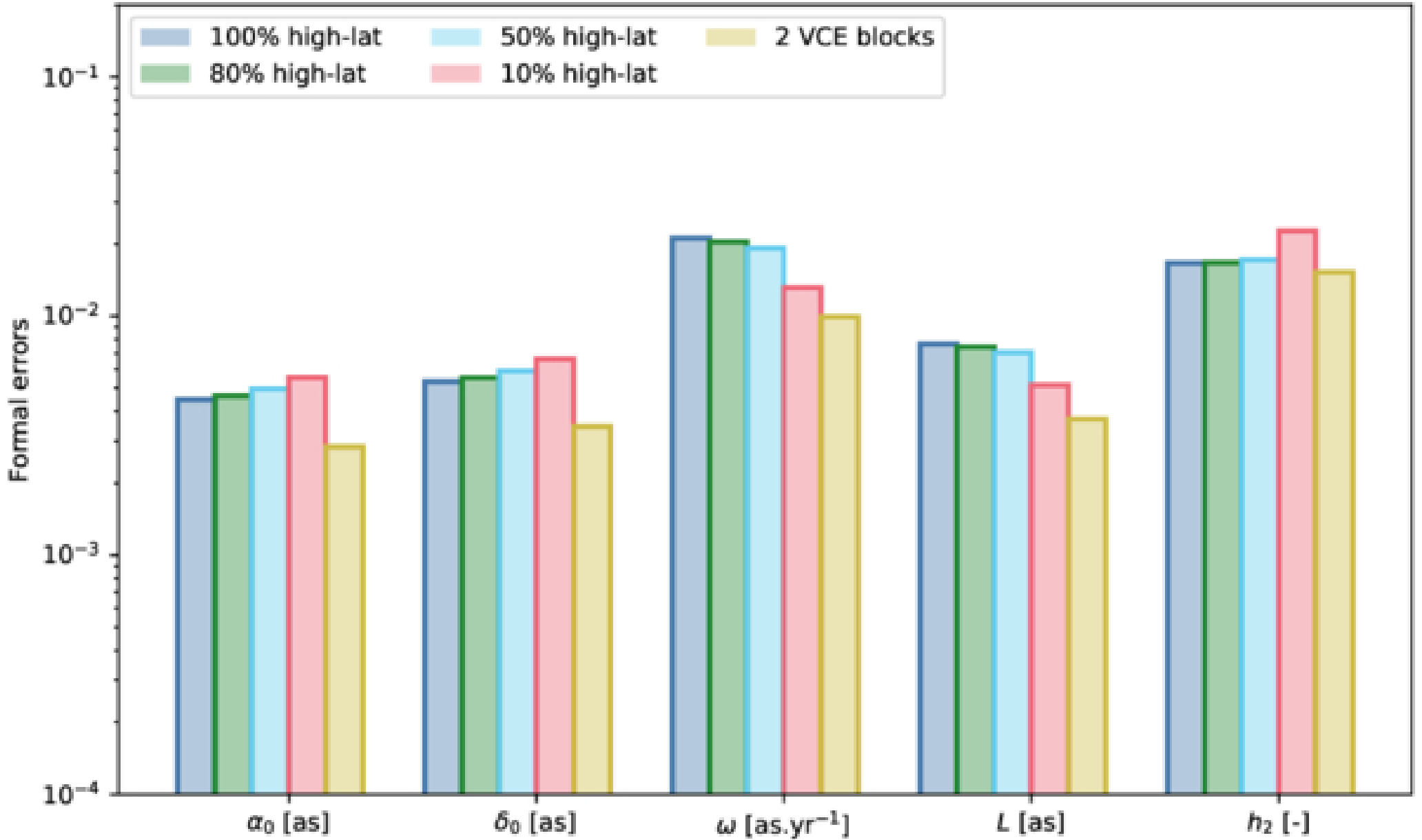
Figure 7. from William Desprats et al 2026 Planet. Sci. J. 7 doi:10.3847/PSJ/ae71c3 https://dx.doi.org/10.3847/PSJ/ae71c3 © 2026. The Author(s). Published by the American Astronomical Society.
