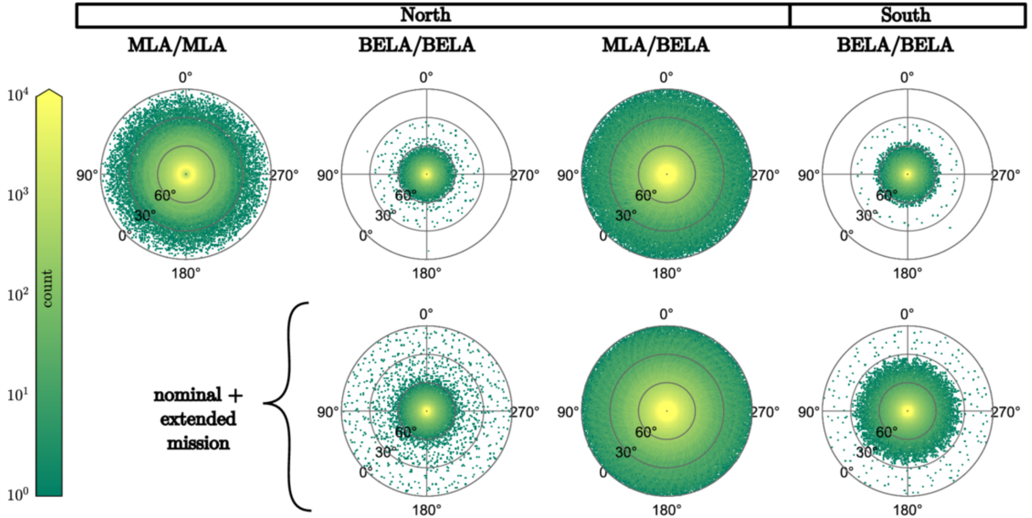
Figure 3. from William Desprats et al 2026 Planet. Sci. J. 7 doi:10.3847/PSJ/ae71c3 https://dx.doi.org/10.3847/PSJ/ae71c3 © 2026. The Author(s). Published by the American Astronomical Society.
