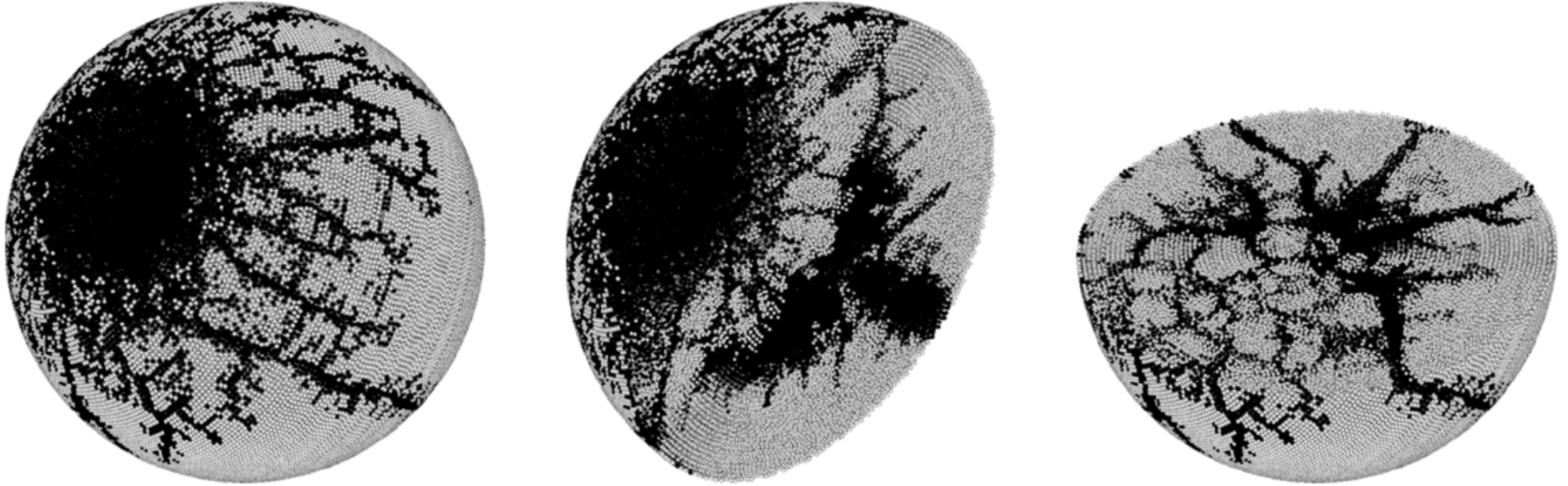
Figure 7. from Sean P. Stokes et al 2026 Planet. Sci. J. 7 doi:10.3847/PSJ/ae71b8 https://dx.doi.org/10.3847/PSJ/ae71b8 © 2026. The Author(s). Published by the American Astronomical Society.
