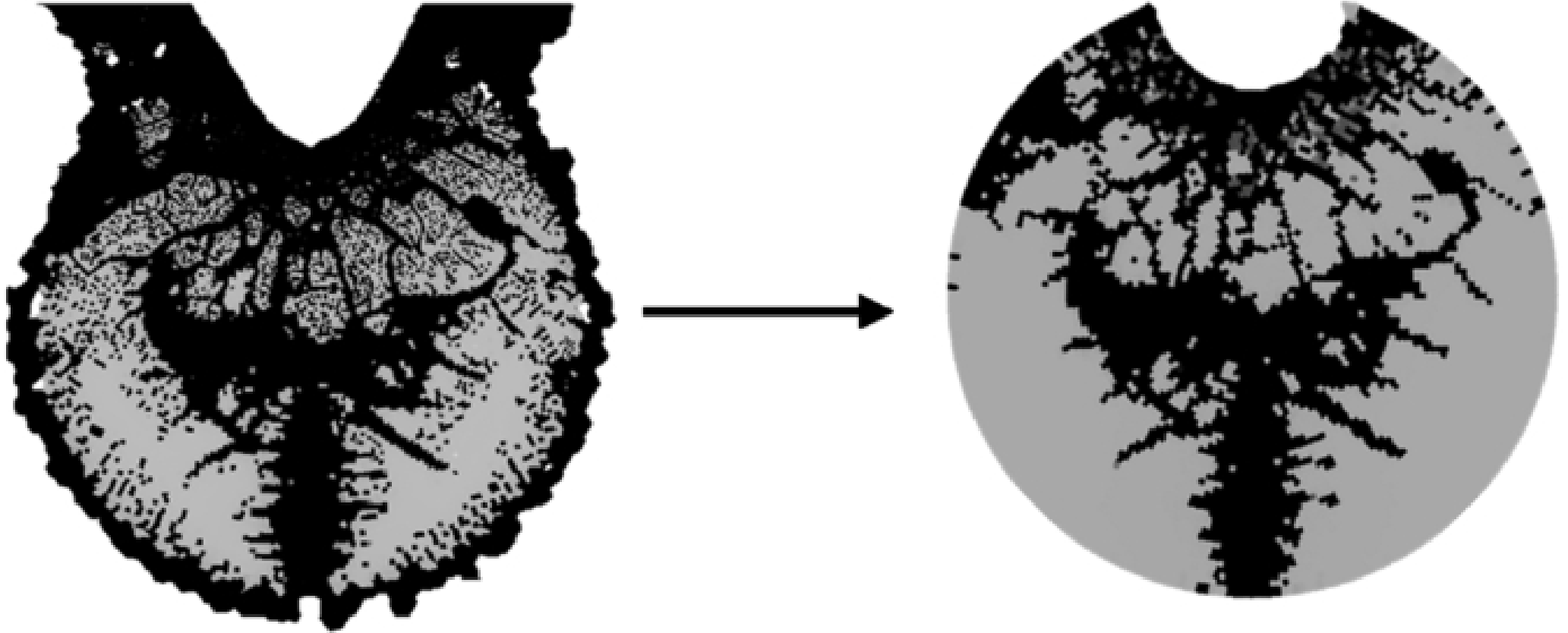
Figure 2. from Sean P. Stokes et al 2026 Planet. Sci. J. 7 doi:10.3847/PSJ/ae71b8 https://dx.doi.org/10.3847/PSJ/ae71b8 © 2026. The Author(s). Published by the American Astronomical Society.
