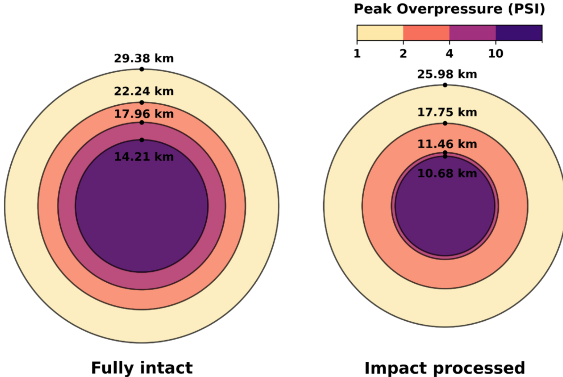
Figure 11. from Sean P. Stokes et al 2026 Planet. Sci. J. 7 doi:10.3847/PSJ/ae71b8 https://dx.doi.org/10.3847/PSJ/ae71b8 © 2026. The Author(s). Published by the American Astronomical Society.
