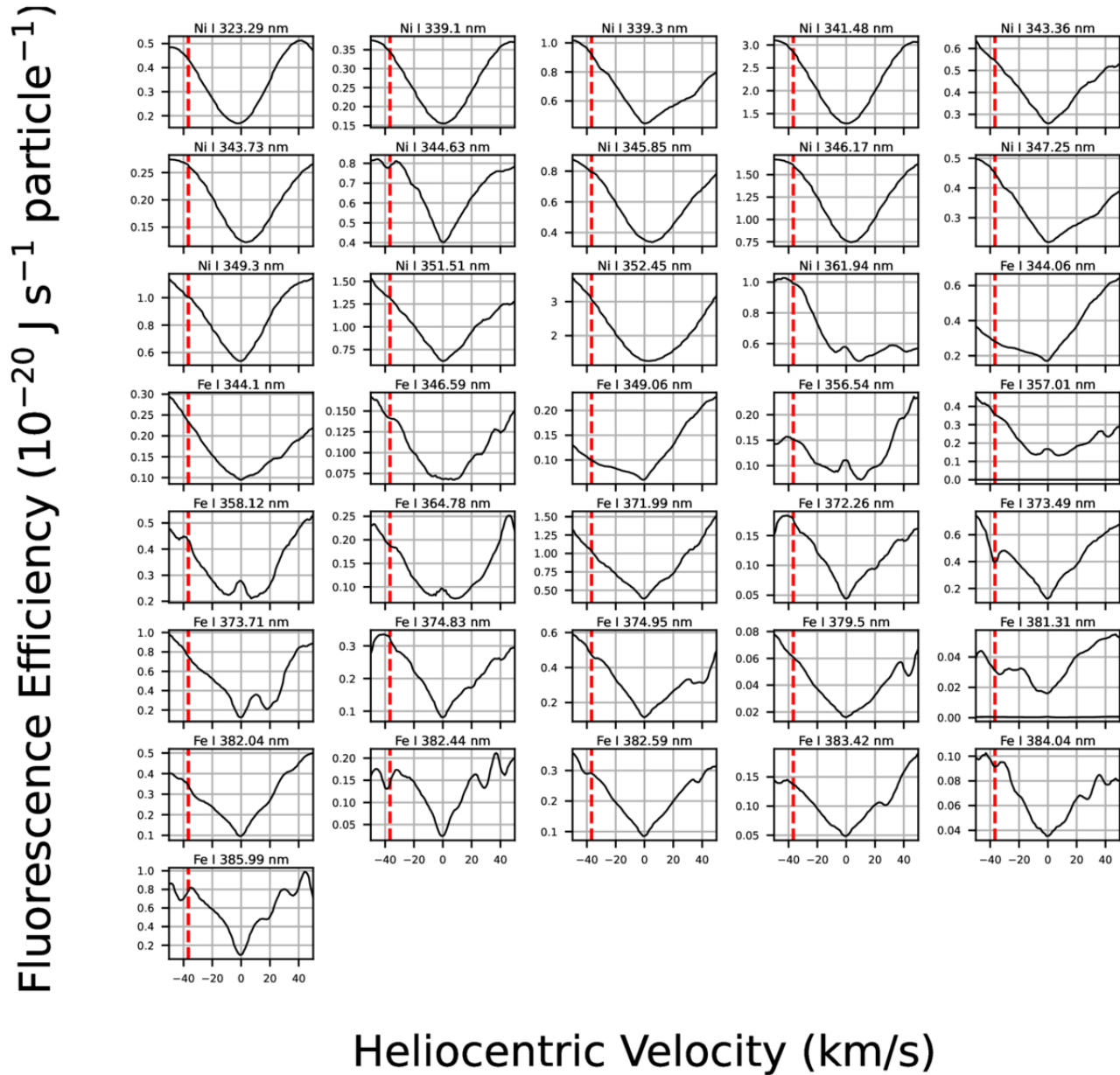
Figure 11. from S. J. Bromley et al 2026 Planet. Sci. J. 7 doi:10.3847/PSJ/ae706d https://dx.doi.org/10.3847/PSJ/ae706d © 2026. The Author(s). Published by the American Astronomical Society.
