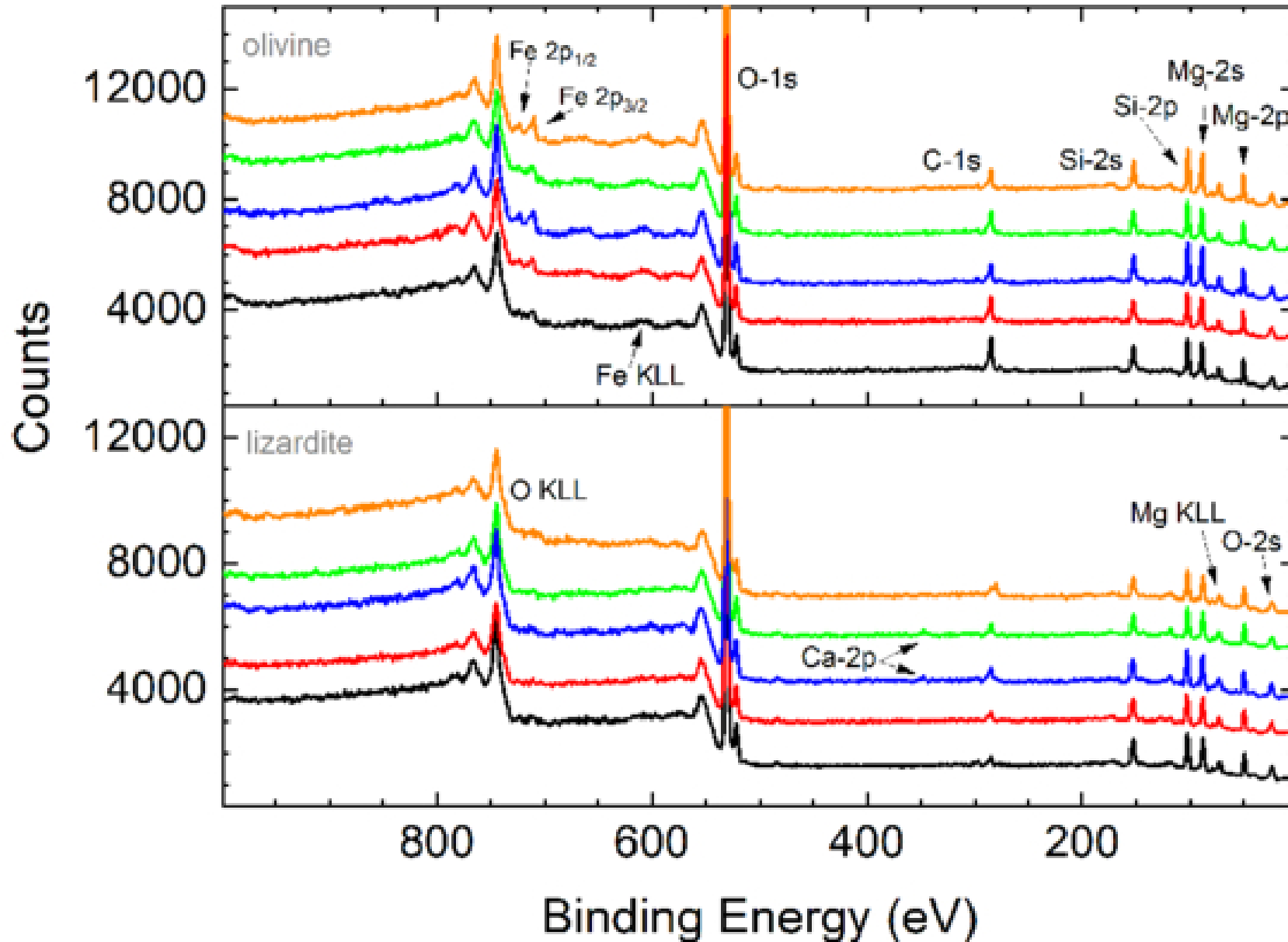
Figure A1. from Nicole M. Ozdowski et al 2026 Planet. Sci. J. 7 doi:10.3847/PSJ/ae6faa https://dx.doi.org/10.3847/PSJ/ae6faa © 2026. The Author(s). Published by the American Astronomical Society.
