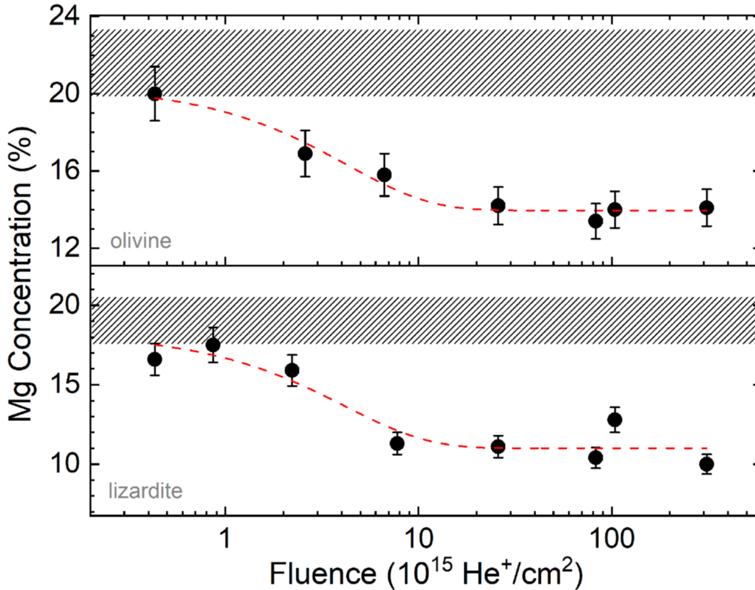
Figure 7. from Nicole M. Ozdowski et al 2026 Planet. Sci. J. 7 doi:10.3847/PSJ/ae6faa https://dx.doi.org/10.3847/PSJ/ae6faa © 2026. The Author(s). Published by the American Astronomical Society.
