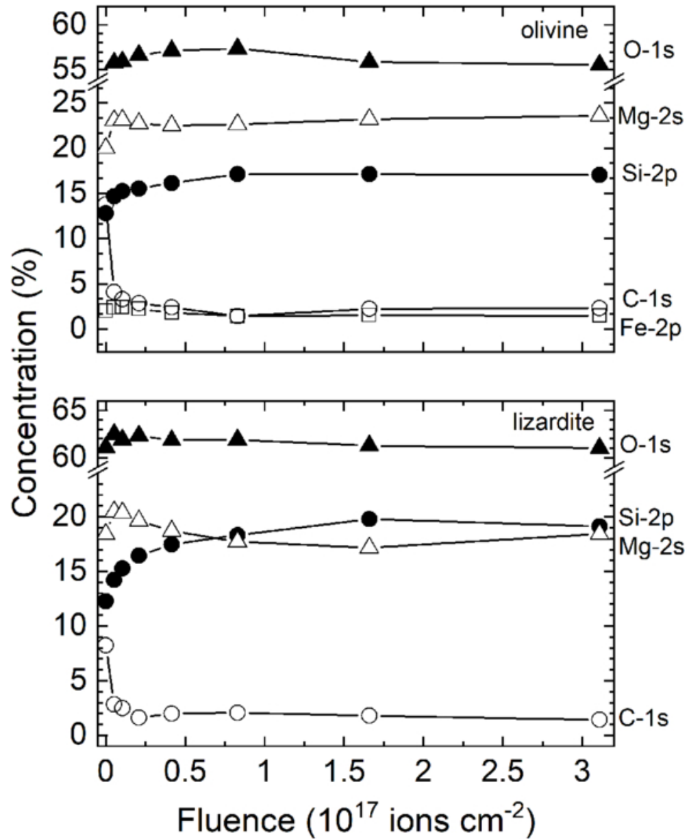
Figure 6. from Nicole M. Ozdowski et al 2026 Planet. Sci. J. 7 doi:10.3847/PSJ/ae6faa https://dx.doi.org/10.3847/PSJ/ae6faa © 2026. The Author(s). Published by the American Astronomical Society.
