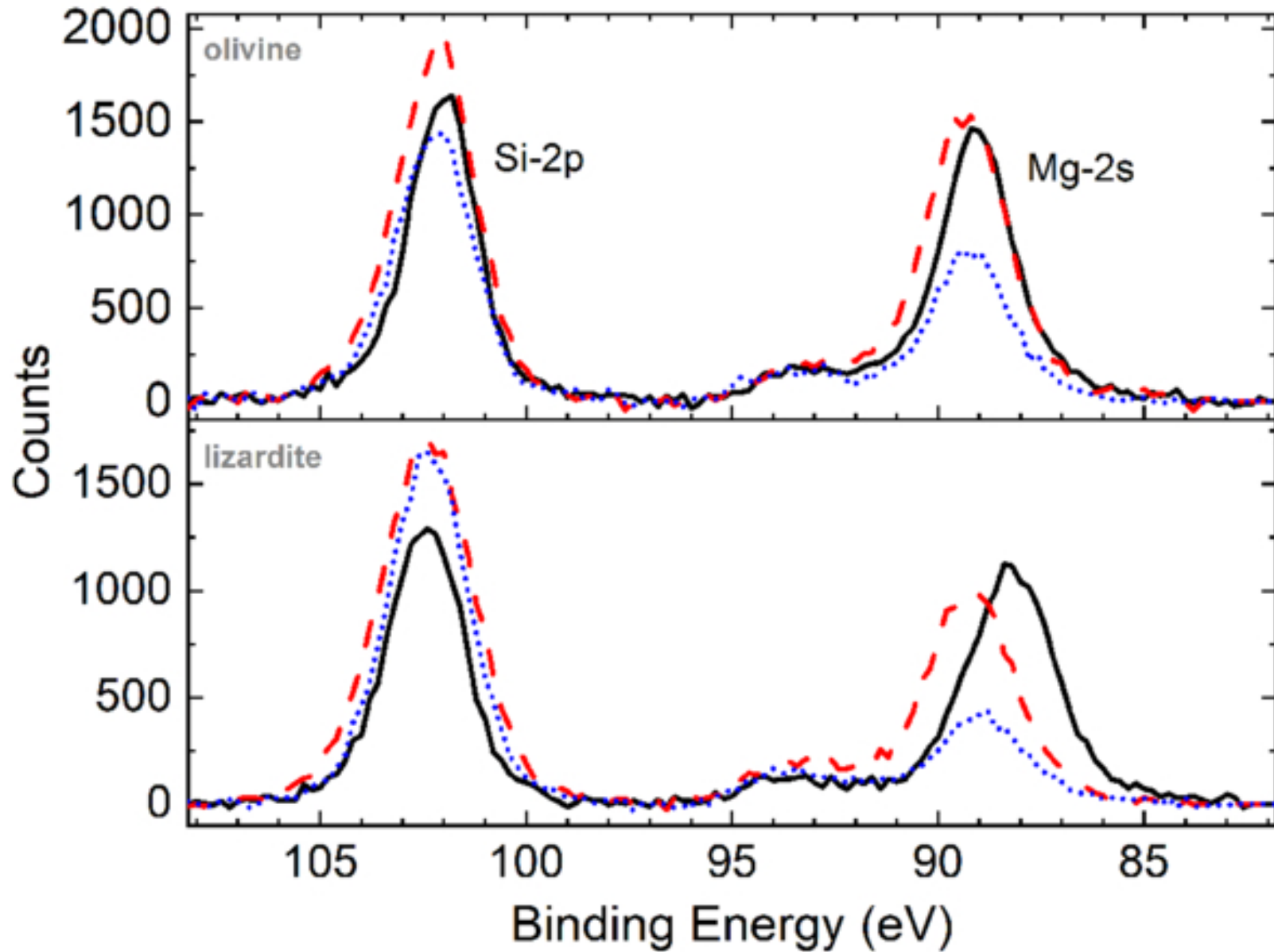
Figure 5. from Nicole M. Ozdowski et al 2026 Planet. Sci. J. 7 doi:10.3847/PSJ/ae6faa https://dx.doi.org/10.3847/PSJ/ae6faa © 2026. The Author(s). Published by the American Astronomical Society.
