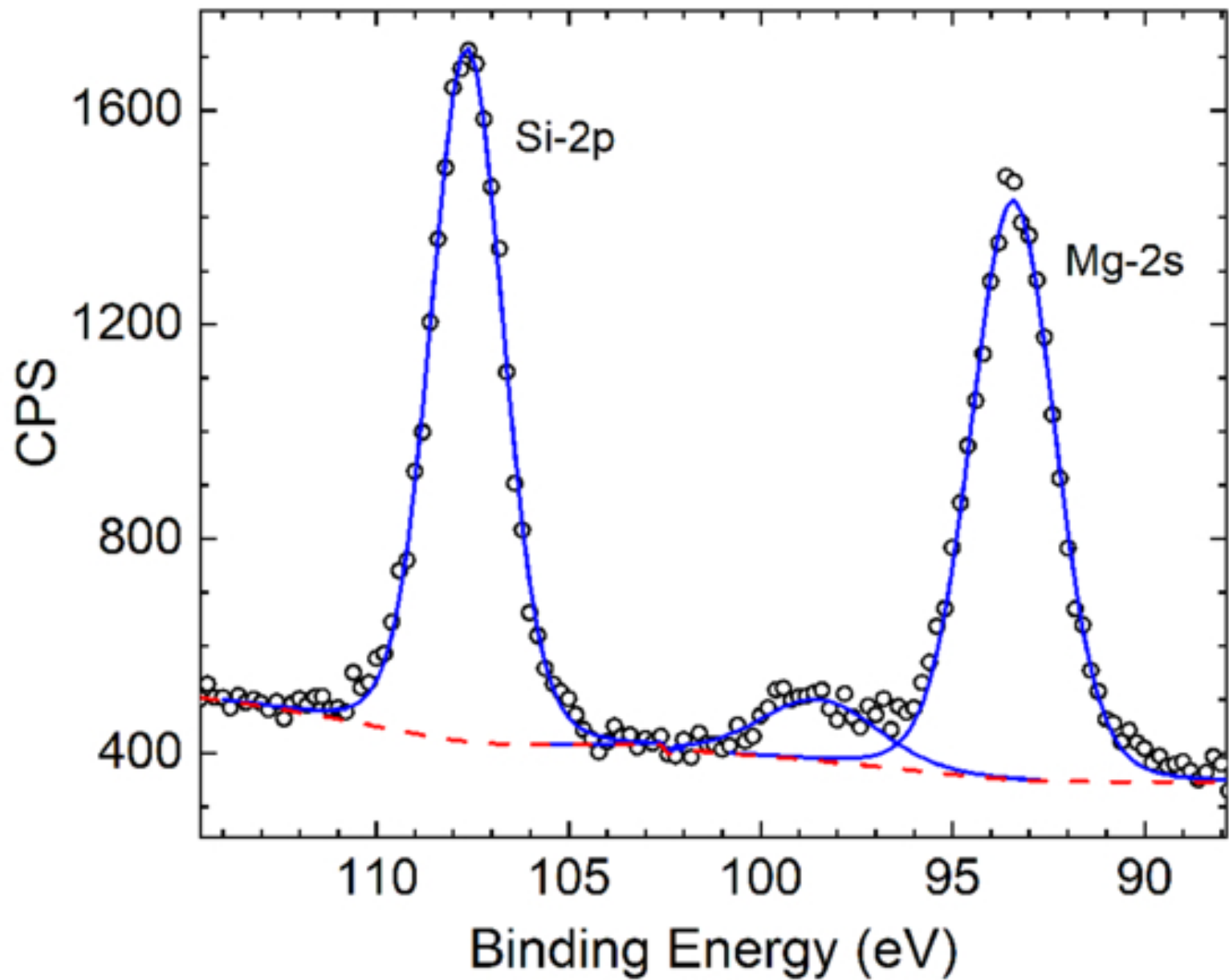
Figure 3. from Nicole M. Ozdowski et al 2026 Planet. Sci. J. 7 doi:10.3847/PSJ/ae6faa https://dx.doi.org/10.3847/PSJ/ae6faa © 2026. The Author(s). Published by the American Astronomical Society.
