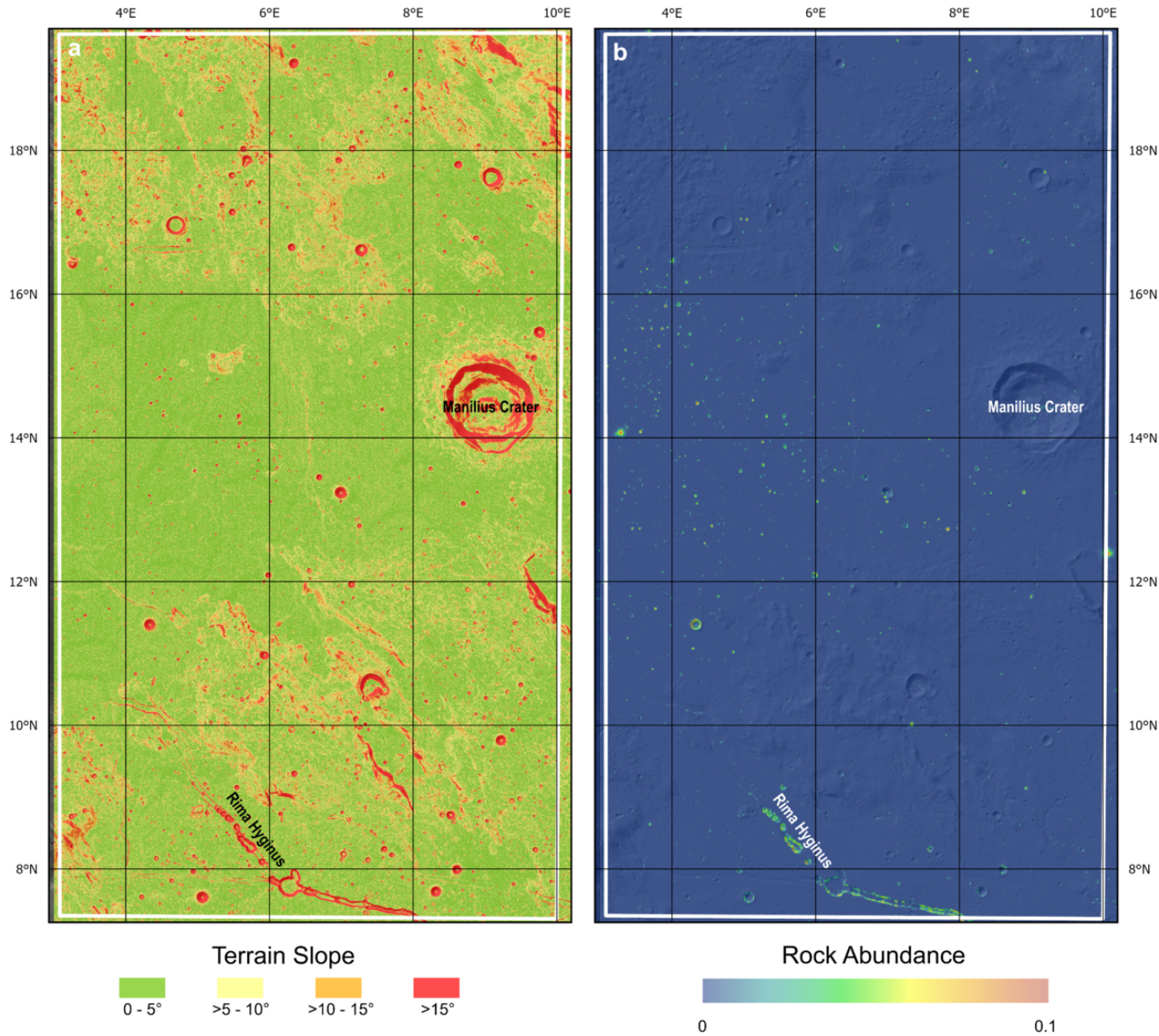
Figure 9. from Astrid Oetting et al 2026 Planet. Sci. J. 7 doi:10.3847/PSJ/ae6fa5 https://dx.doi.org/10.3847/PSJ/ae6fa5 © 2026. The Author(s). Published by the American Astronomical Society.
