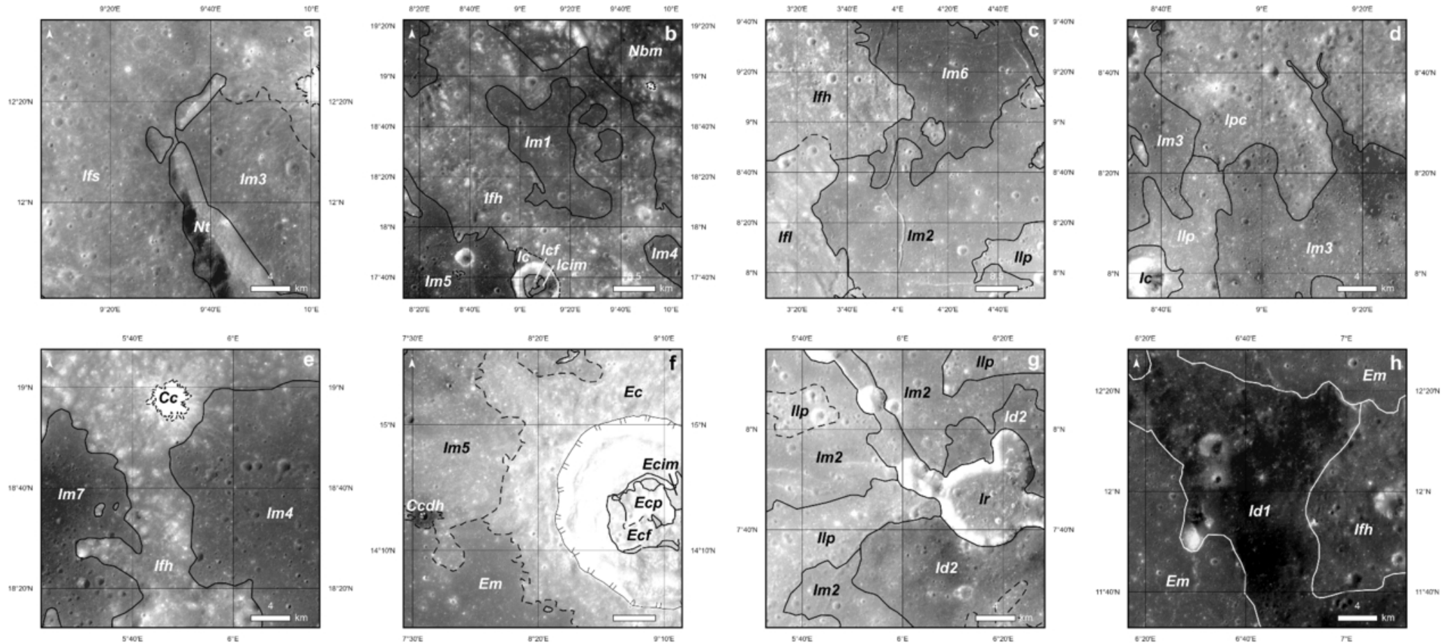
Figure 3. from Astrid Oetting et al 2026 Planet. Sci. J. 7 doi:10.3847/PSJ/ae6fa5 https://dx.doi.org/10.3847/PSJ/ae6fa5 © 2026. The Author(s). Published by the American Astronomical Society.
