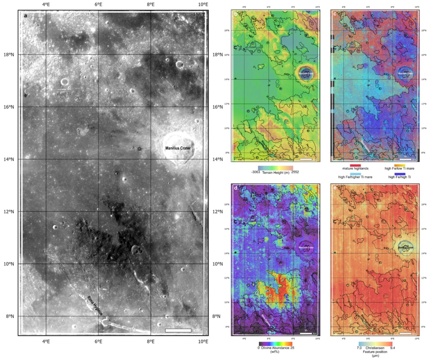
Figure 1. from Astrid Oetting et al 2026 Planet. Sci. J. 7 doi:10.3847/PSJ/ae6fa5 https://dx.doi.org/10.3847/PSJ/ae6fa5 © 2026. The Author(s). Published by the American Astronomical Society.
