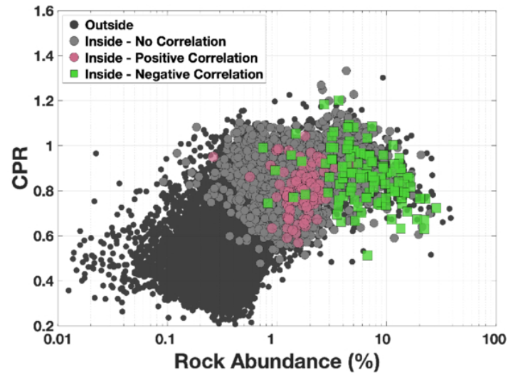
Figure 6. from Edgard G. Rivera-Valentín et al 2026 Planet. Sci. J. 7 doi:10.3847/PSJ/ae6fa4 https://dx.doi.org/10.3847/PSJ/ae6fa4 © 2026. The Author(s). Published by the American Astronomical Society.
