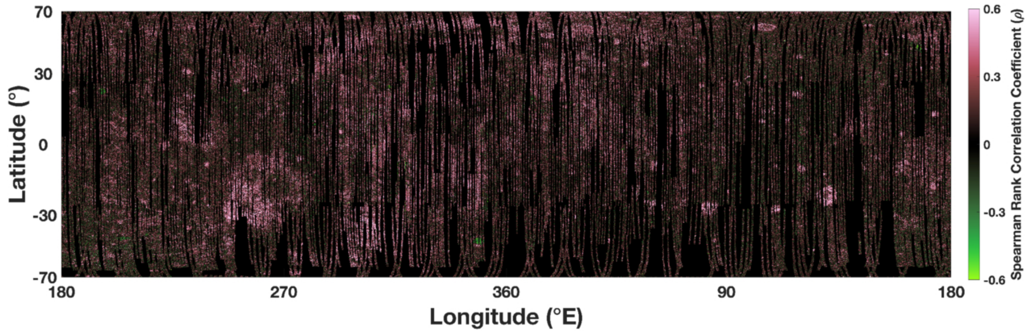
Figure 4. from Edgard G. Rivera-Valentín et al 2026 Planet. Sci. J. 7 doi:10.3847/PSJ/ae6fa4 https://dx.doi.org/10.3847/PSJ/ae6fa4 © 2026. The Author(s). Published by the American Astronomical Society.
