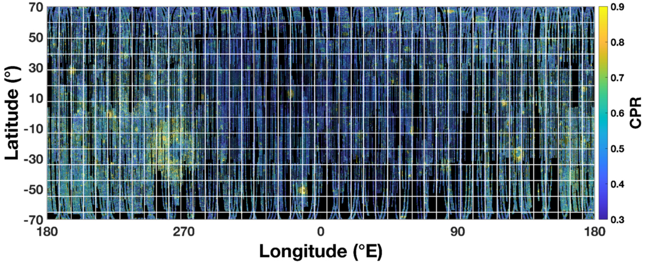
Figure 1. from Edgard G. Rivera-Valentín et al 2026 Planet. Sci. J. 7 doi:10.3847/PSJ/ae6fa4 https://dx.doi.org/10.3847/PSJ/ae6fa4 © 2026. The Author(s). Published by the American Astronomical Society.
