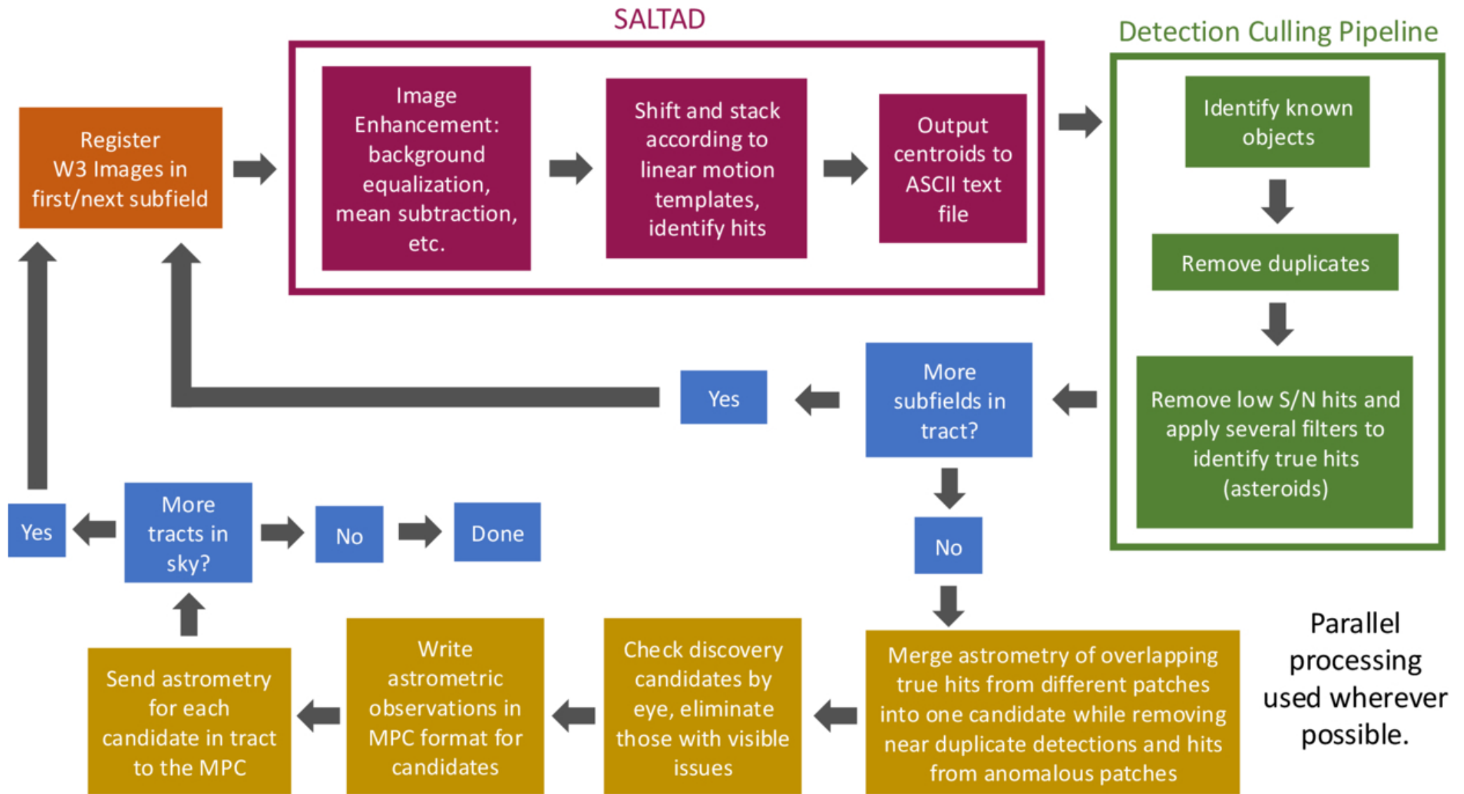
Figure 4. from Emerson A. Whittaker and Jean-Luc Margot 2026 Planet. Sci. J. 7 doi:10.3847/PSJ/ae6fa1 https://dx.doi.org/10.3847/PSJ/ae6fa1 © 2026. The Author(s). Published by the American Astronomical Society.
