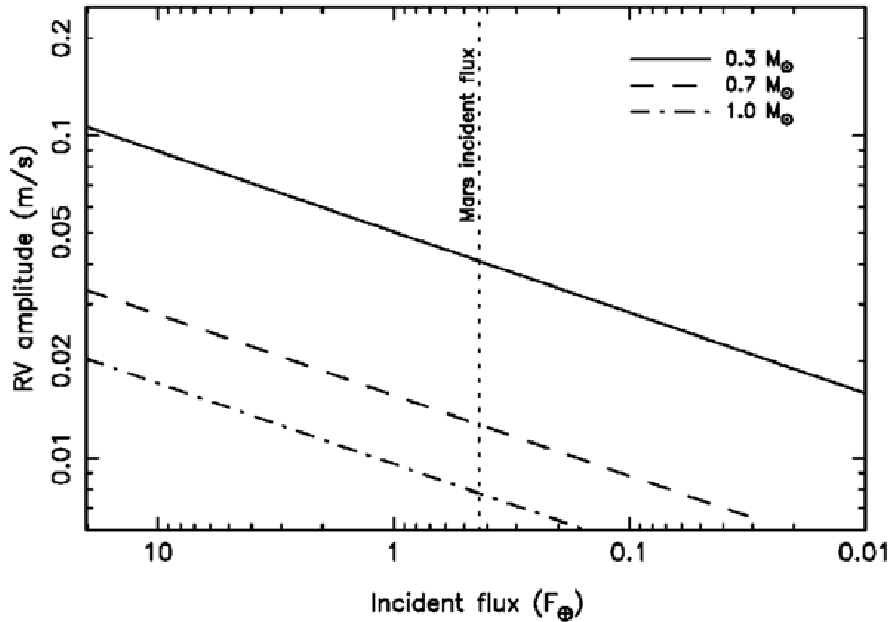
Figure 3. from Stephen R. Kane et al 2026 Planet. Sci. J. 7 doi:10.3847/PSJ/ae6f00 https://dx.doi.org/10.3847/PSJ/ae6f00 © 2026. The Author(s). Published by the American Astronomical Society.
