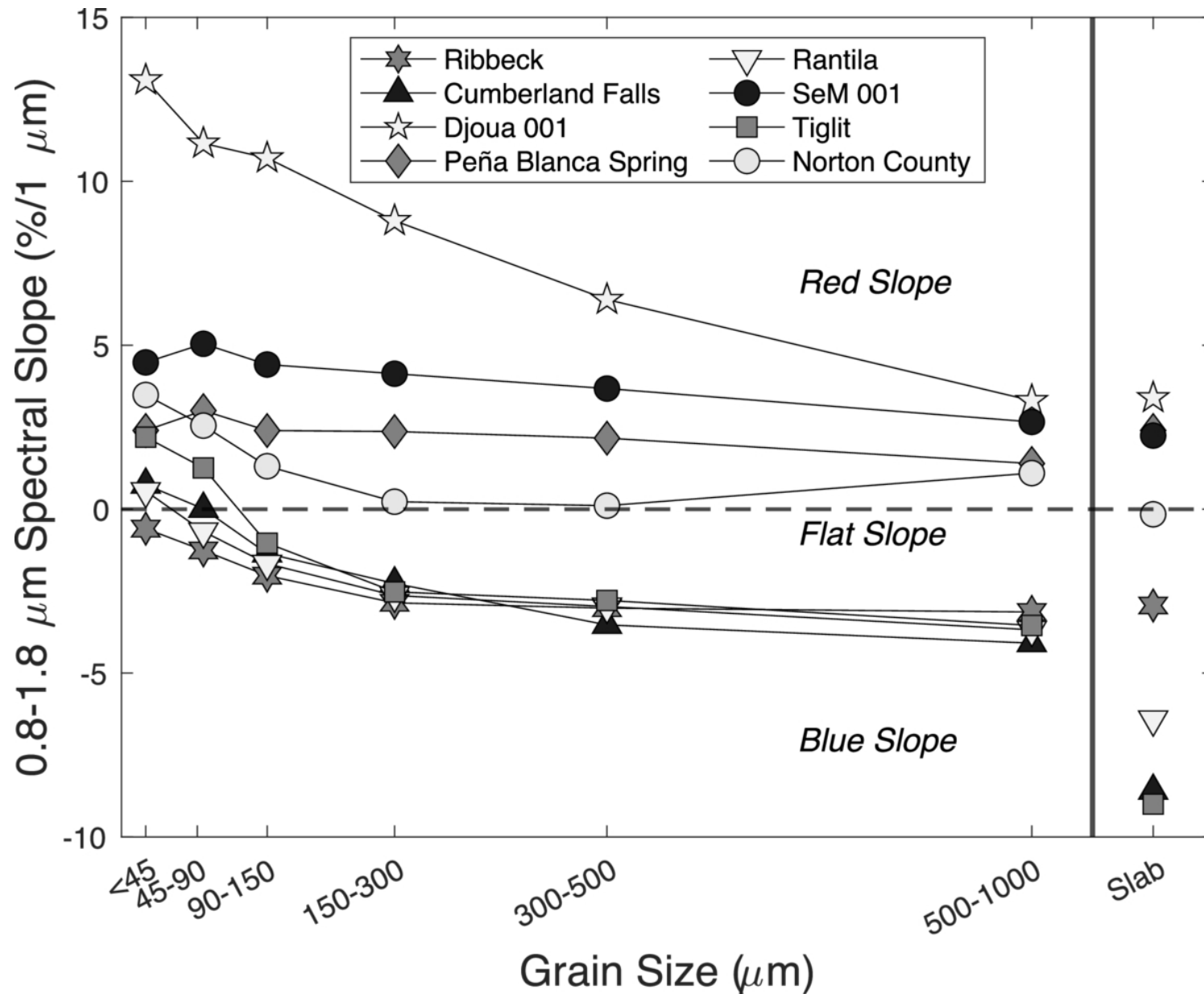
Figure 9. from David C. Cantillo et al 2026 Planet. Sci. J. 7 doi:10.3847/PSJ/ae6db2 https://dx.doi.org/10.3847/PSJ/ae6db2 © 2026. The Author(s). Published by the American Astronomical Society.
