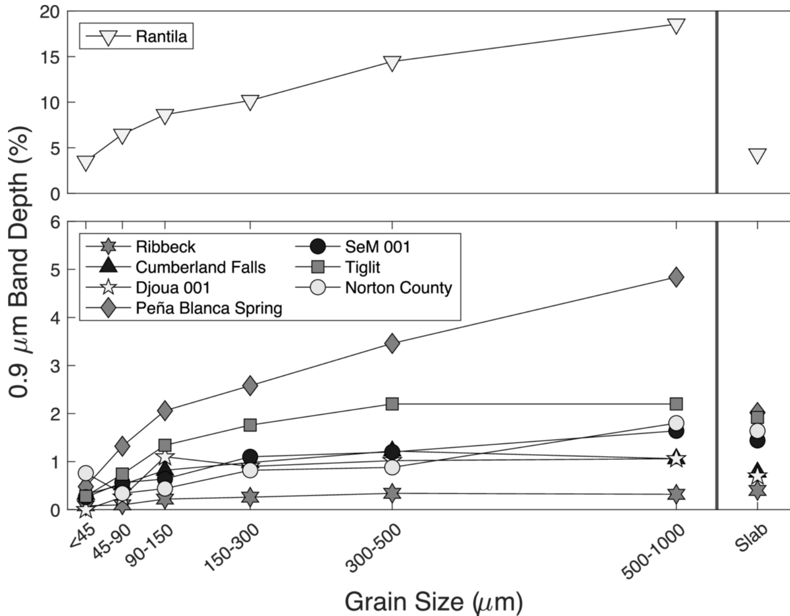
Figure 7. from David C. Cantillo et al 2026 Planet. Sci. J. 7 doi:10.3847/PSJ/ae6db2 https://dx.doi.org/10.3847/PSJ/ae6db2 © 2026. The Author(s). Published by the American Astronomical Society.
