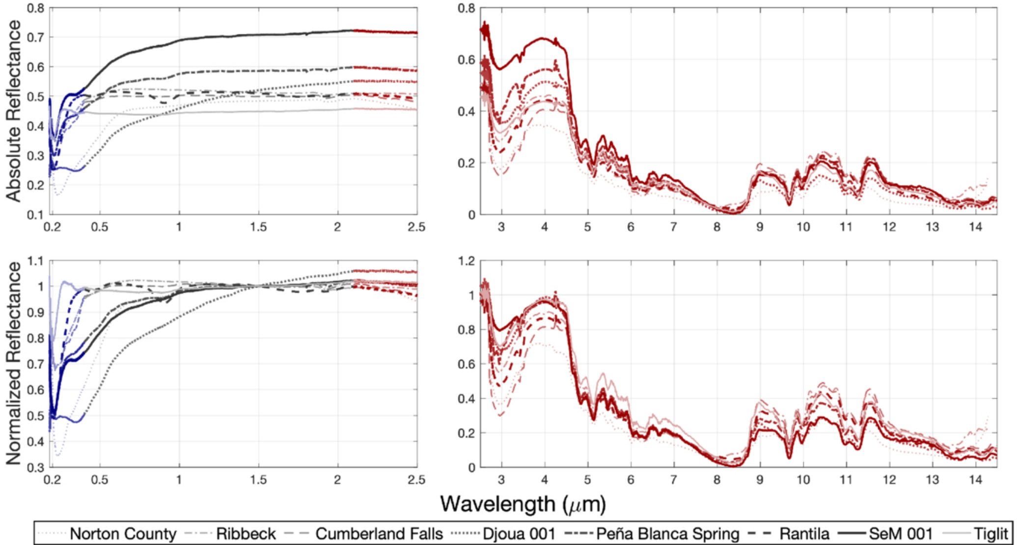
Figure 4. from David C. Cantillo et al 2026 Planet. Sci. J. 7 doi:10.3847/PSJ/ae6db2 https://dx.doi.org/10.3847/PSJ/ae6db2 © 2026. The Author(s). Published by the American Astronomical Society.
