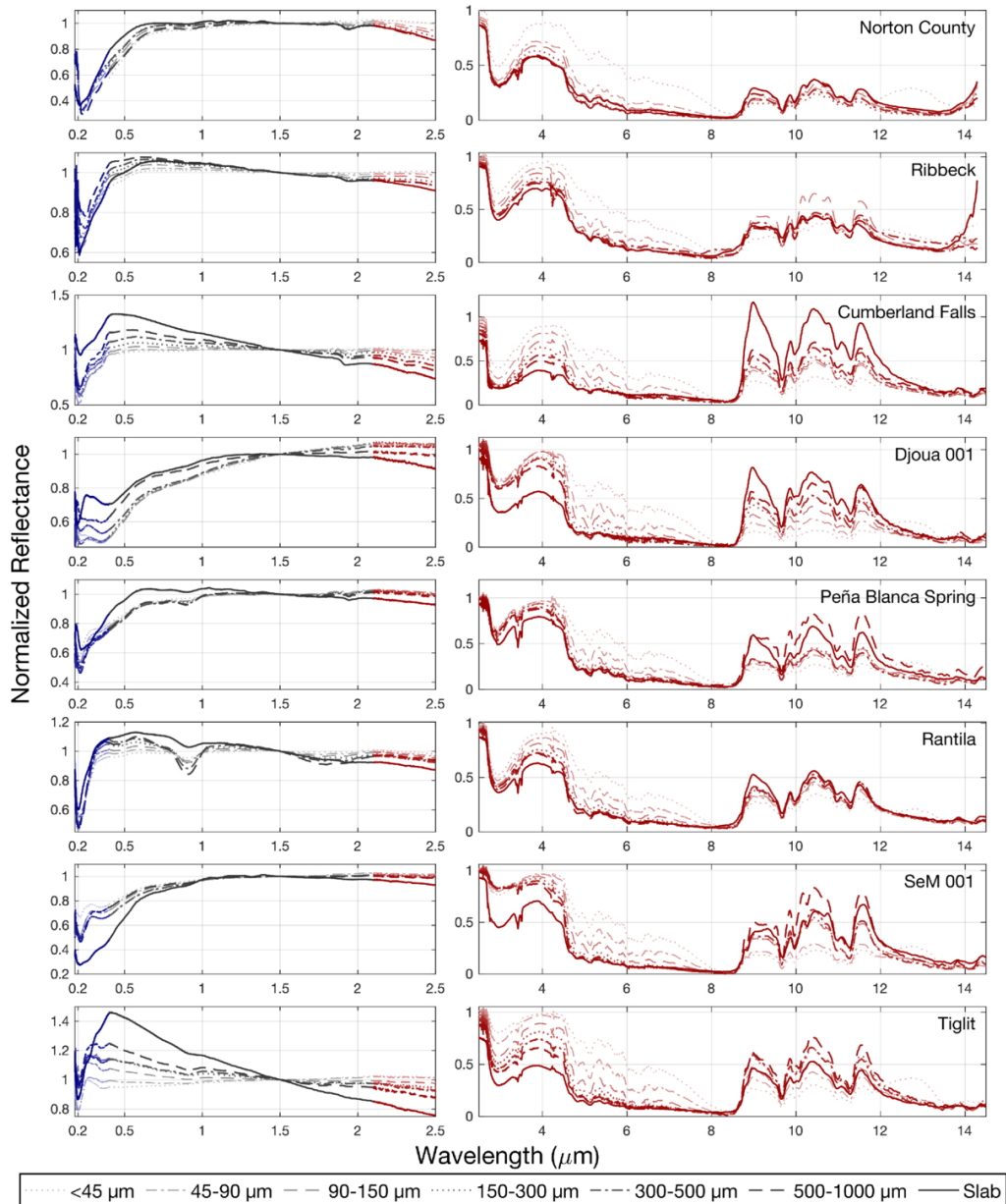
Figure 3. from David C. Cantillo et al 2026 Planet. Sci. J. 7 doi:10.3847/PSJ/ae6db2 https://dx.doi.org/10.3847/PSJ/ae6db2 © 2026. The Author(s). Published by the American Astronomical Society.
