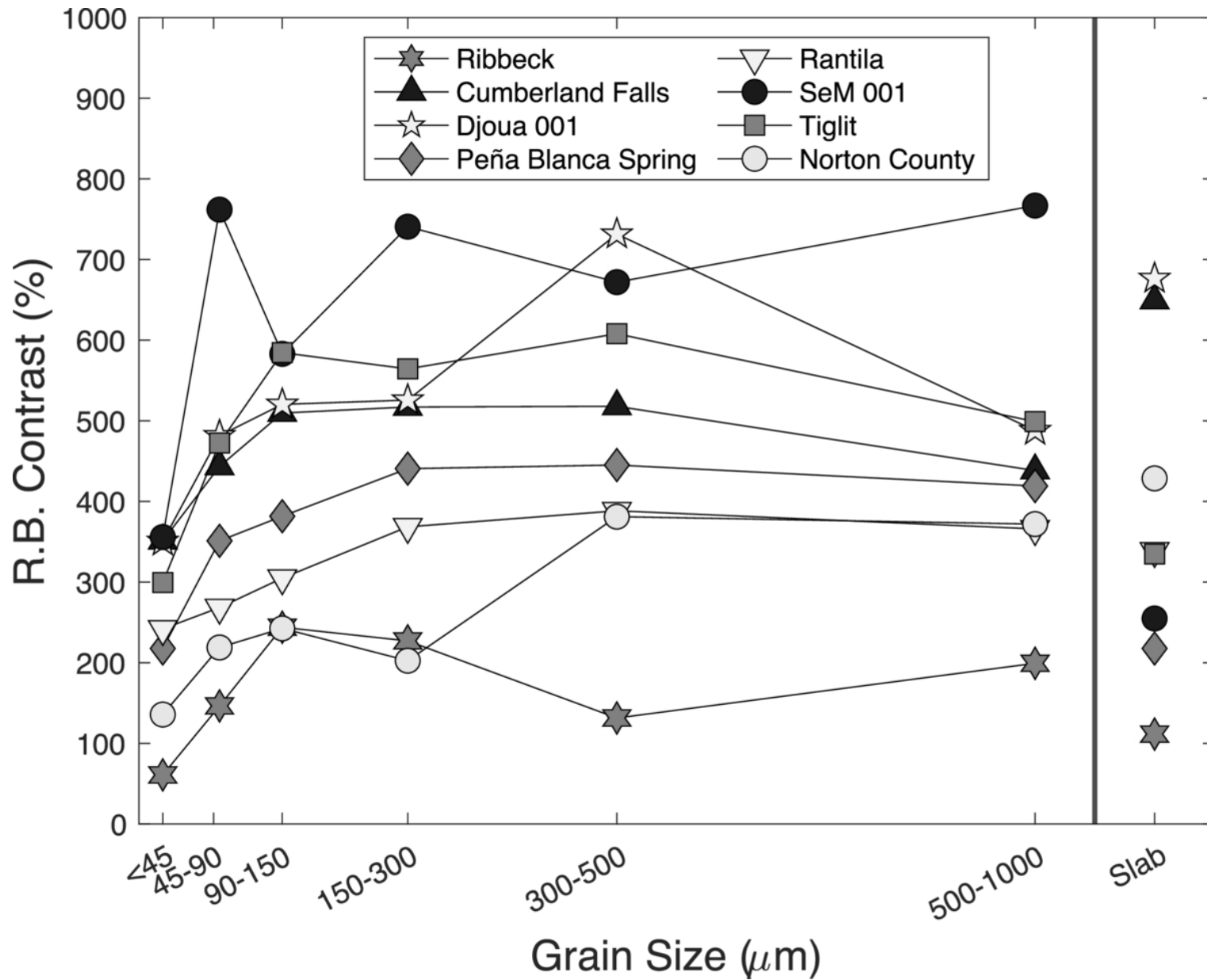
Figure 12. from David C. Cantillo et al 2026 Planet. Sci. J. 7 doi:10.3847/PSJ/ae6db2 https://dx.doi.org/10.3847/PSJ/ae6db2 © 2026. The Author(s). Published by the American Astronomical Society.
