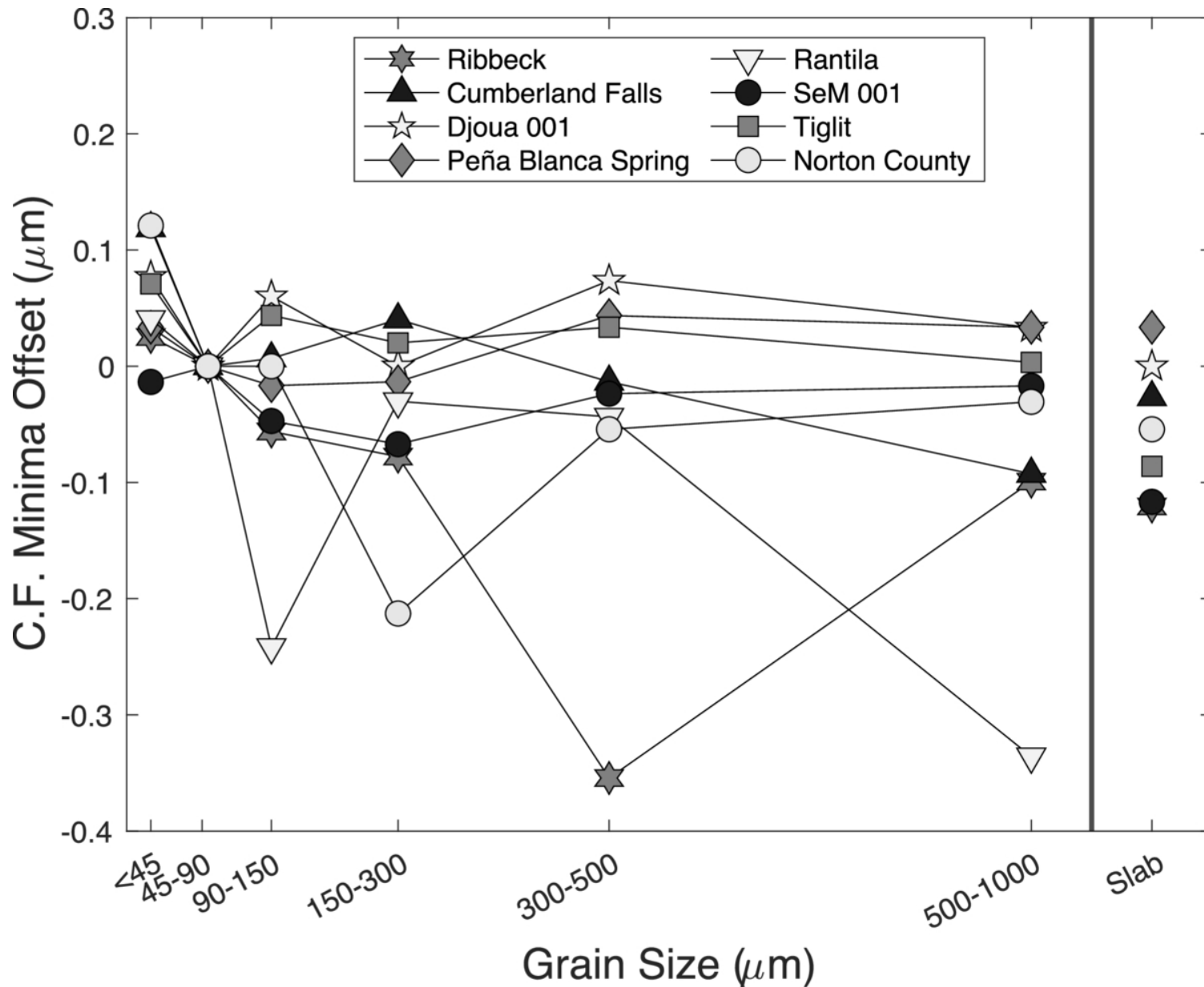
Figure 10. from David C. Cantillo et al 2026 Planet. Sci. J. 7 doi:10.3847/PSJ/ae6db2 https://dx.doi.org/10.3847/PSJ/ae6db2 © 2026. The Author(s). Published by the American Astronomical Society.
