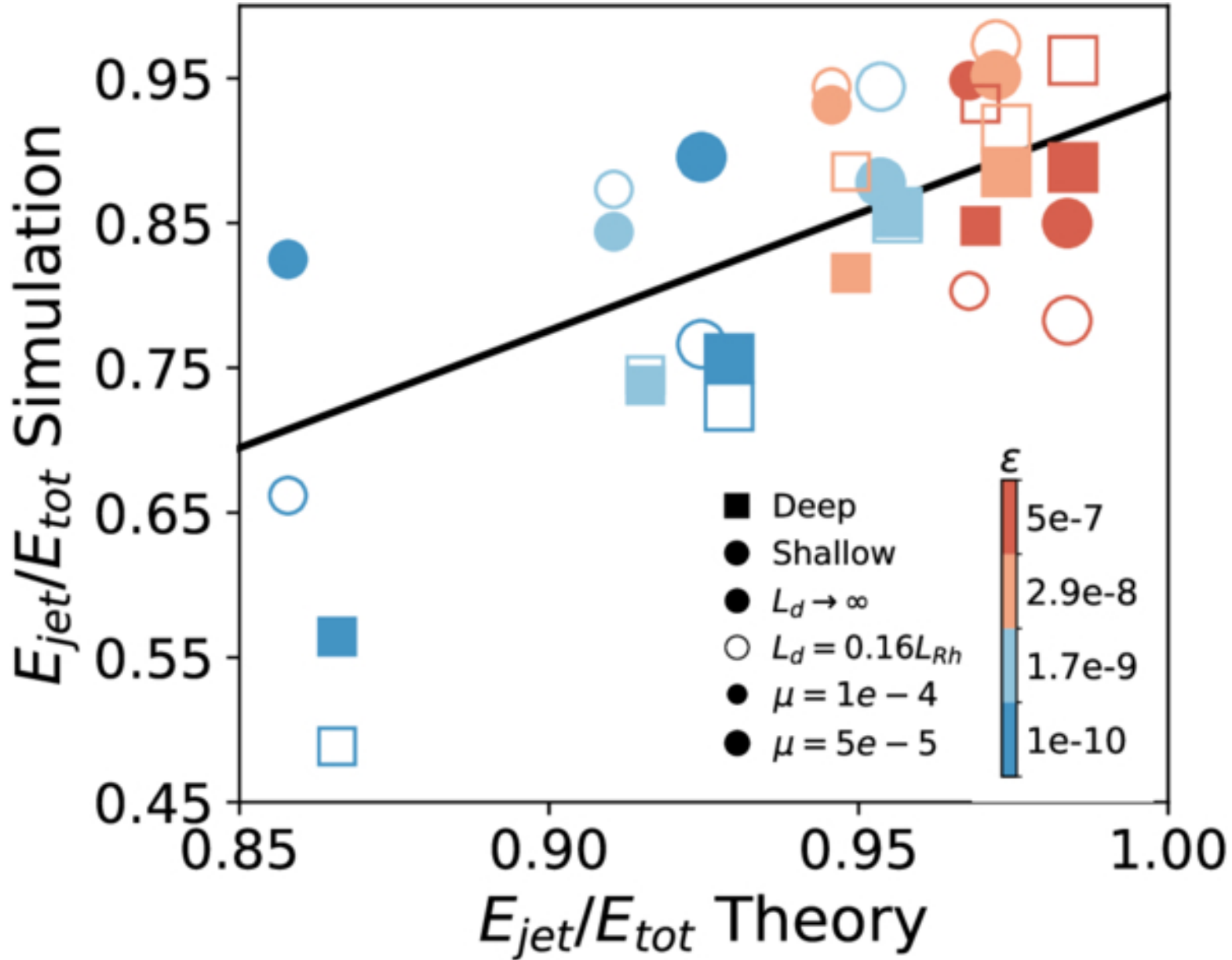
Figure 9. from Yaoxuan Zeng et al 2026 Planet. Sci. J. 7 doi:10.3847/PSJ/ae6da7 https://dx.doi.org/10.3847/PSJ/ae6da7 © 2026. The Author(s). Published by the American Astronomical Society.
