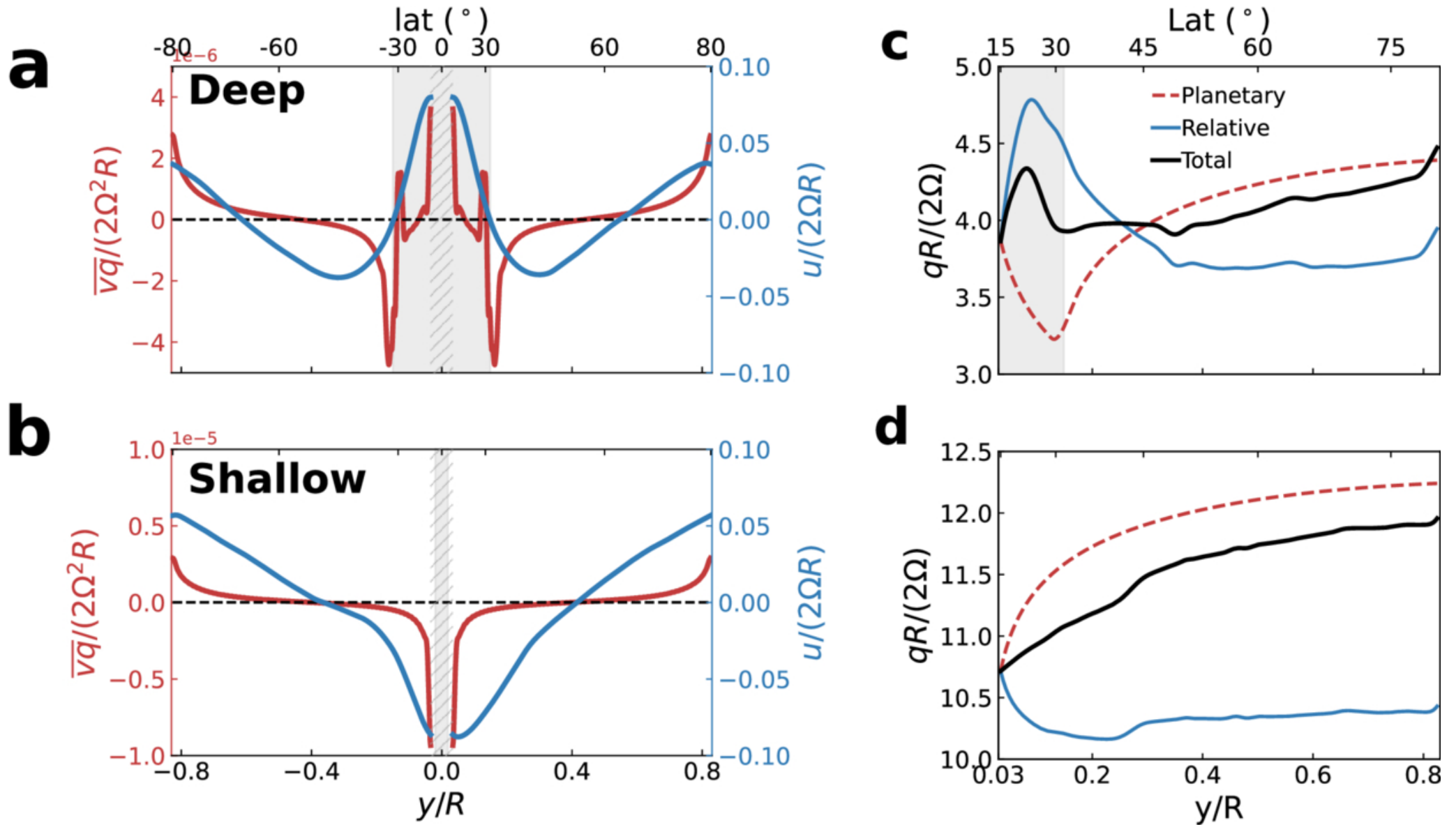
Figure 4. from Yaoxuan Zeng et al 2026 Planet. Sci. J. 7 doi:10.3847/PSJ/ae6da7 https://dx.doi.org/10.3847/PSJ/ae6da7 © 2026. The Author(s). Published by the American Astronomical Society.
