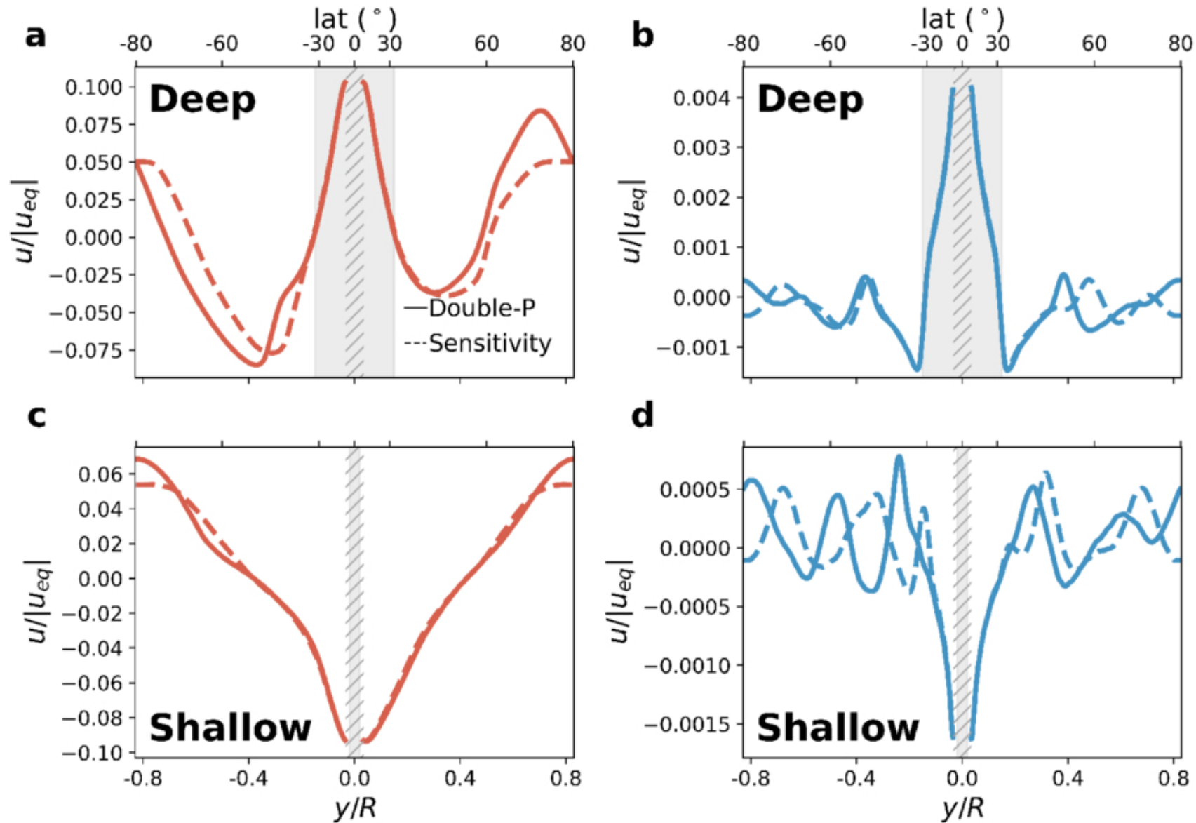
Figure 11. from Yaoxuan Zeng et al 2026 Planet. Sci. J. 7 doi:10.3847/PSJ/ae6da7 https://dx.doi.org/10.3847/PSJ/ae6da7 © 2026. The Author(s). Published by the American Astronomical Society.
