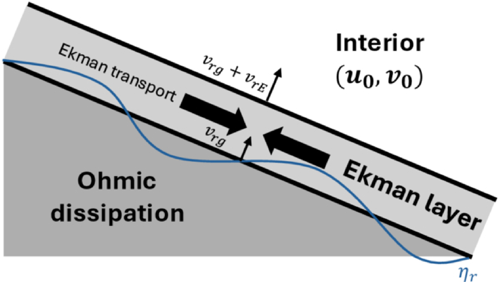
Figure 10. from Yaoxuan Zeng et al 2026 Planet. Sci. J. 7 doi:10.3847/PSJ/ae6da7 https://dx.doi.org/10.3847/PSJ/ae6da7 © 2026. The Author(s). Published by the American Astronomical Society.
